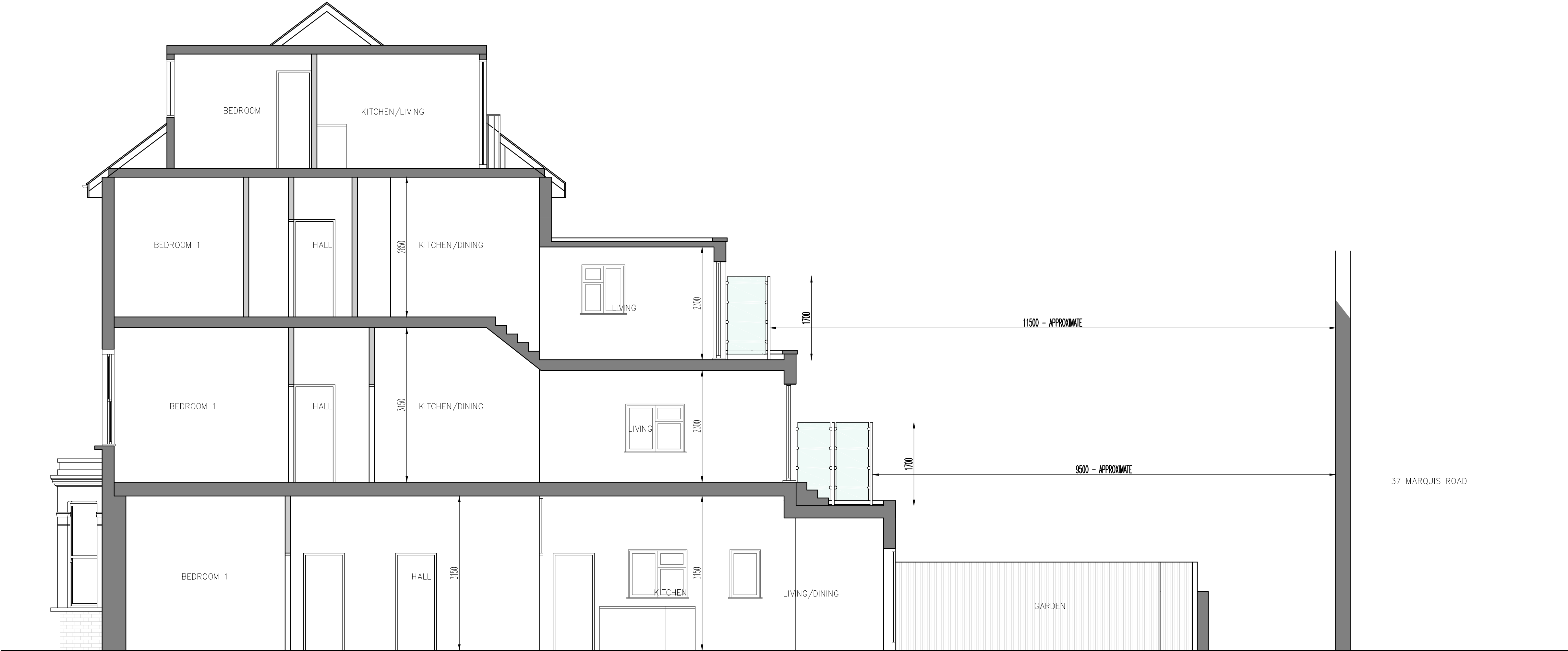
SECTION A-A – PROPOSED
