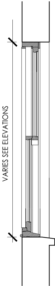
TRADITIONAL SASH WINDOW (WITH WINDOW HORNS)
