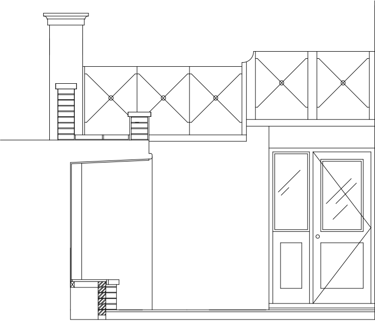
Ext Basement Section-BB
