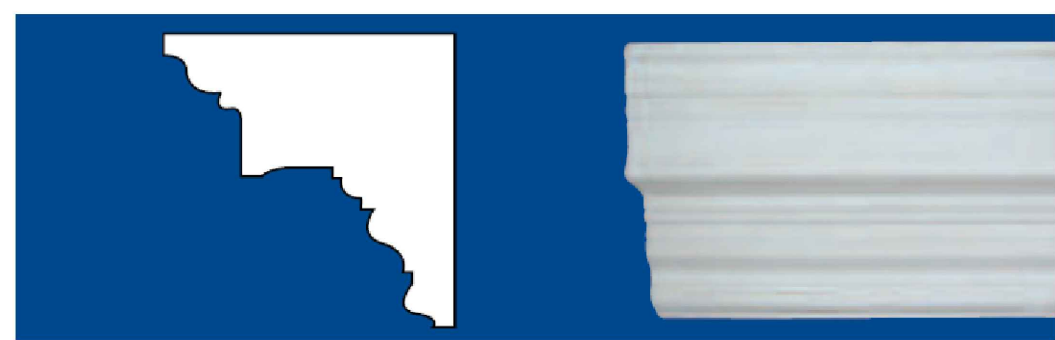
9. CN89 - Depth (215mm) x Projection (220mm) (G- Double height space)
