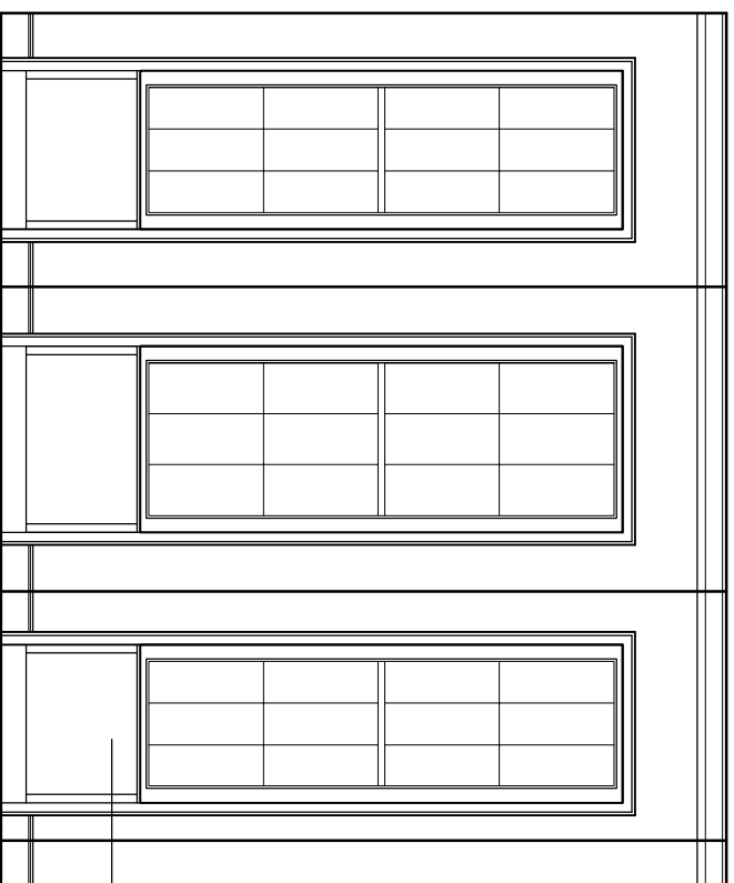
Existing Radiator Casing Elevation
