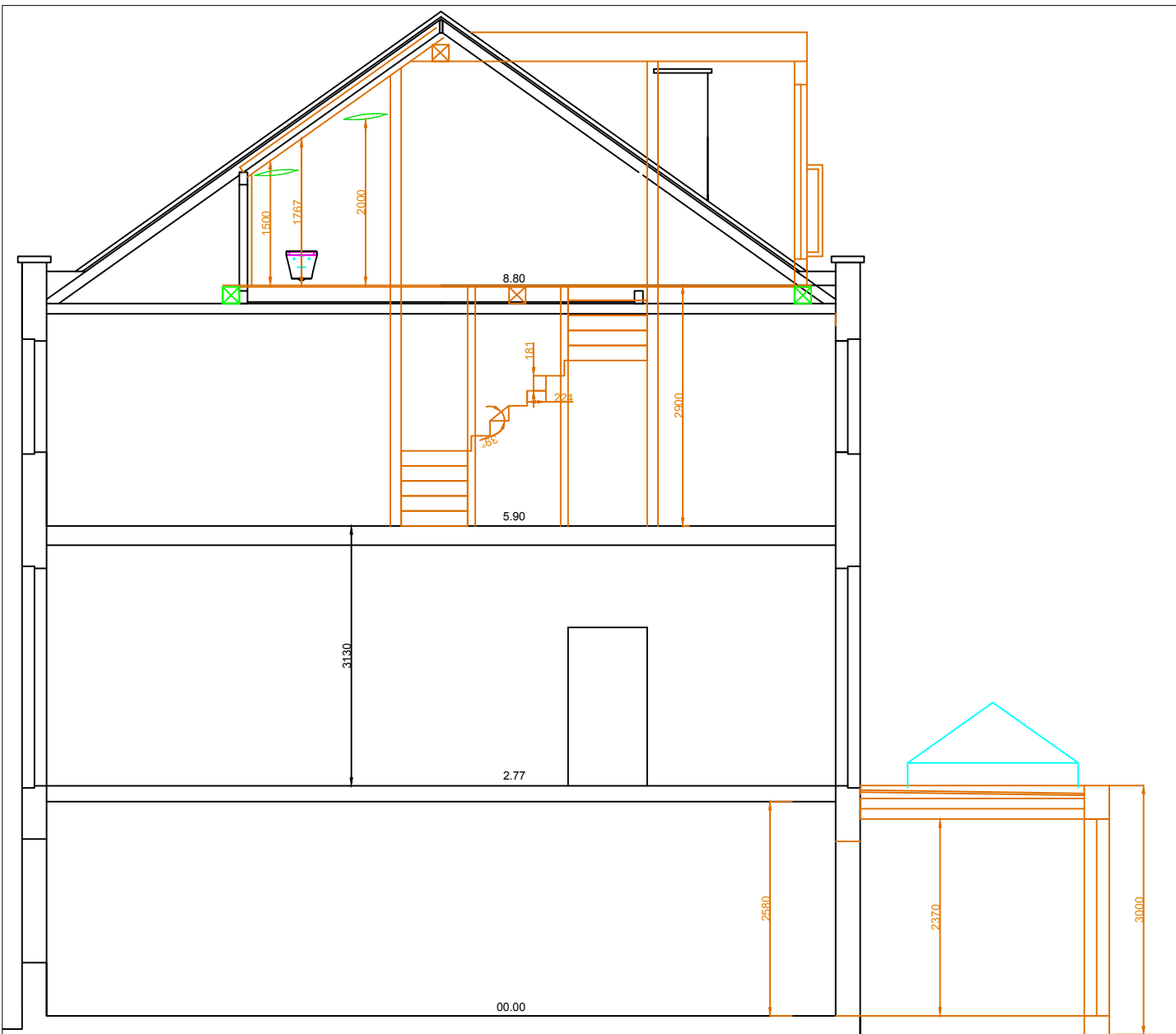
SECTION BB
