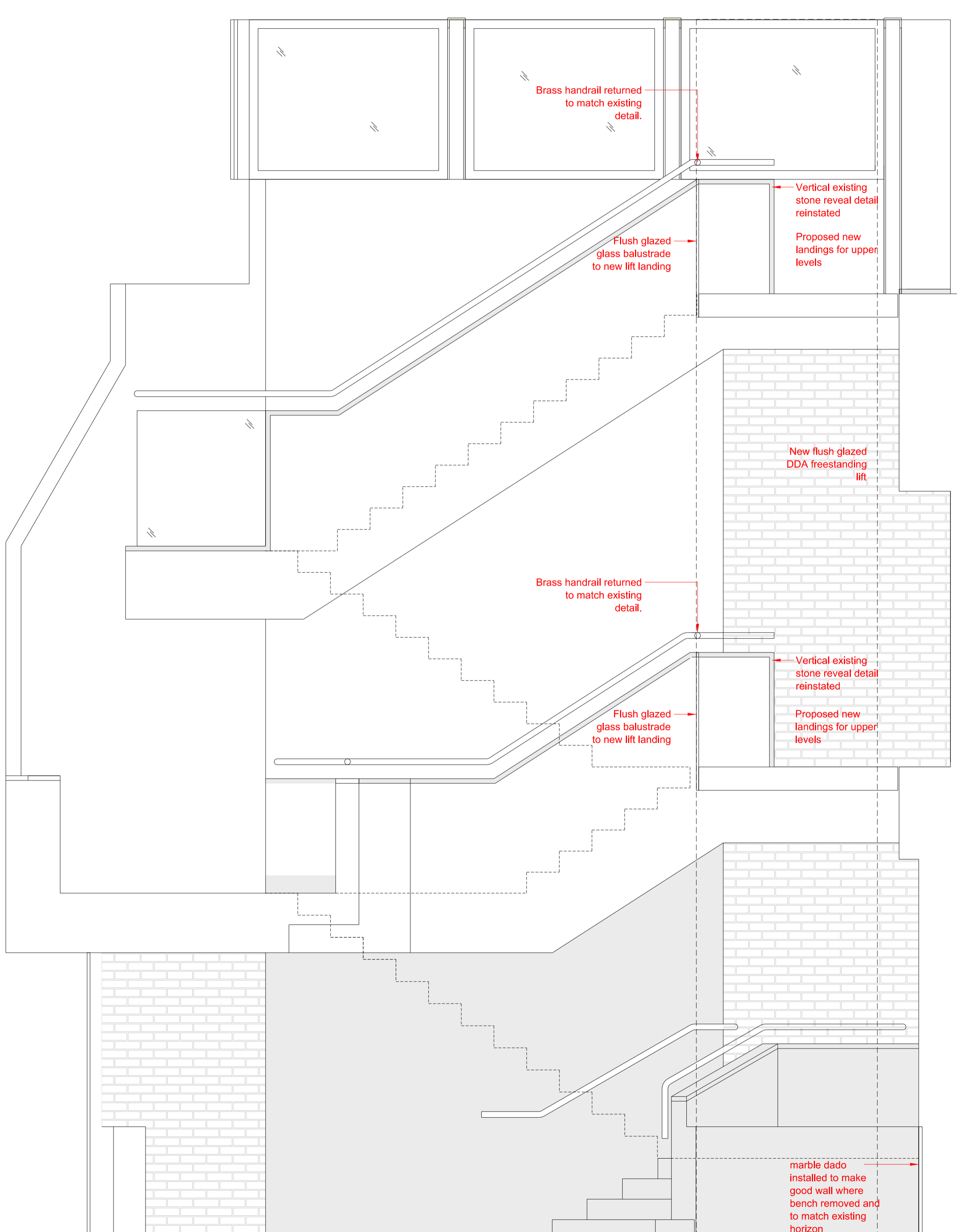
A PROPOSED SECTION AA 1:25 @ A1
