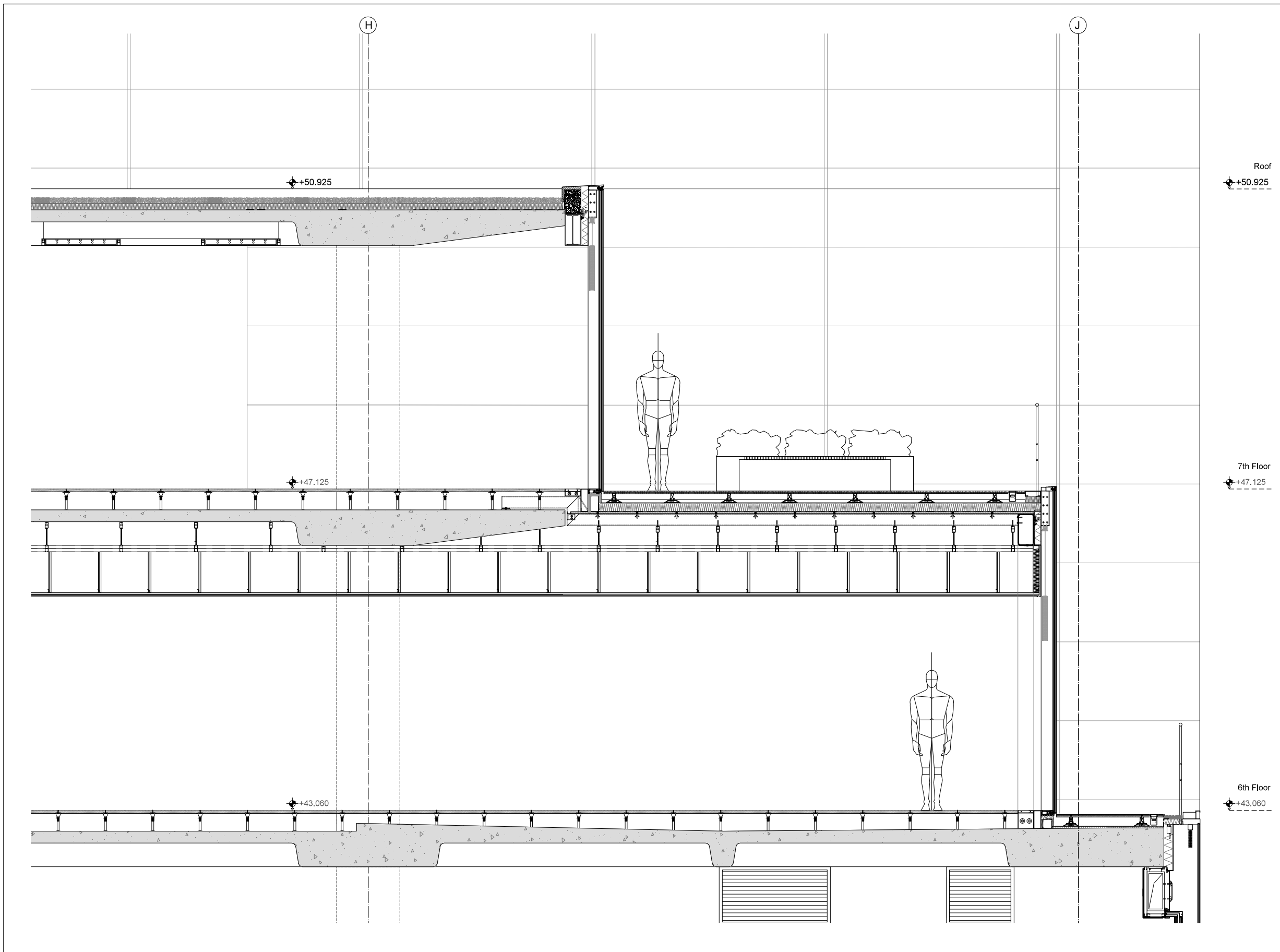
01 Existing Sixth and Seventh Floor Section Detail
