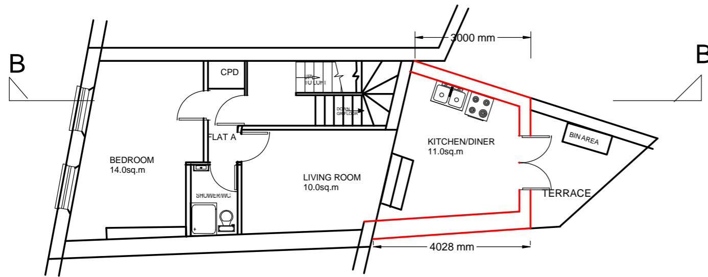
PROPOSED REAR EXTENSION AT FIRST FLOOR-FLAT A
