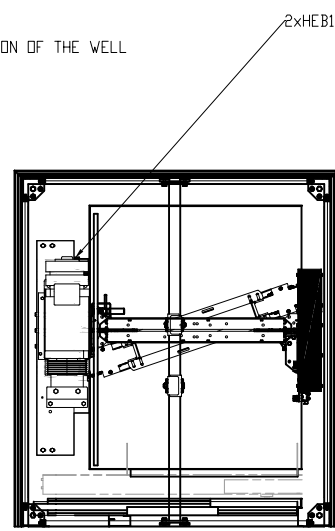
SECTION B-B
