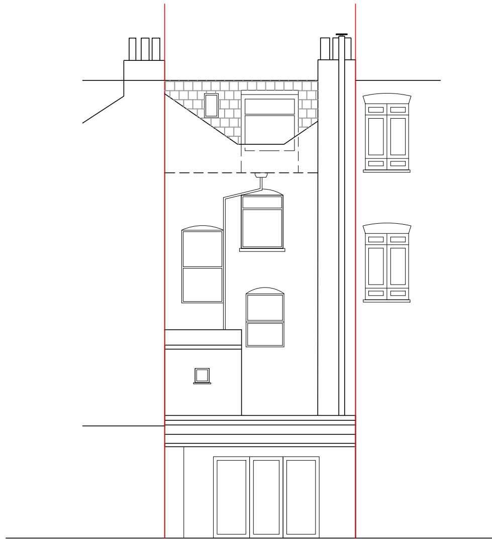
REAR ELAVATION
