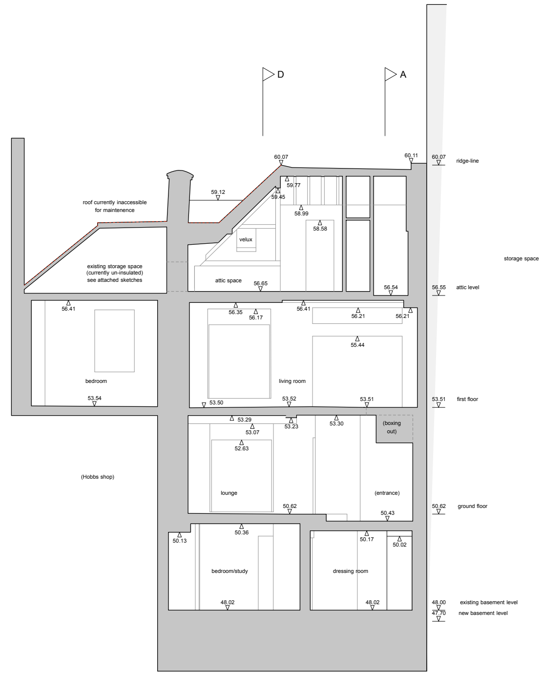
Section BB - As Existing
