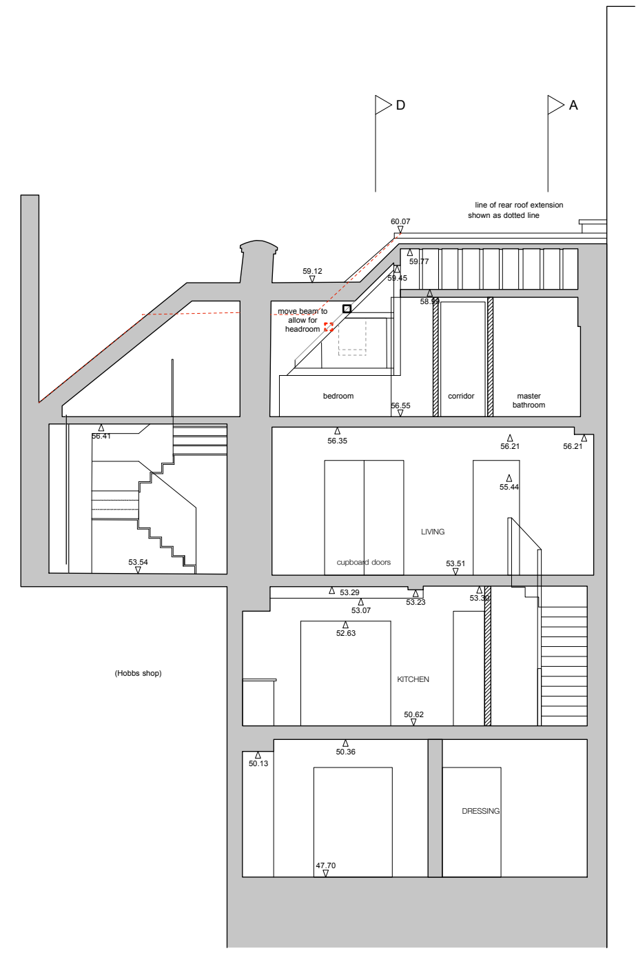
Section BB - As Proposed
