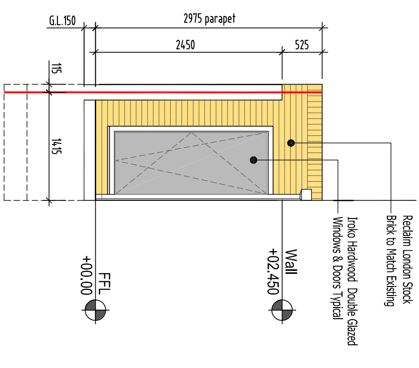
04. Proposed Rear Elevation
