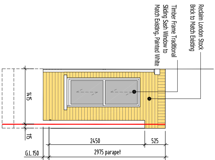
02. Proposed Front Elevation
