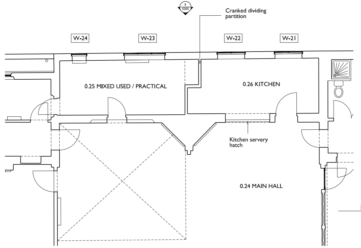
1 Ground floor plan 0105 Scale 1:100
