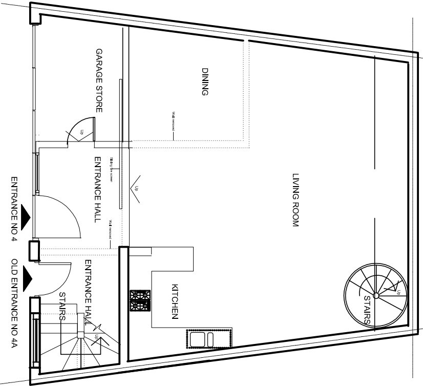
GROUND FLOOR PLAN PROPOSED
