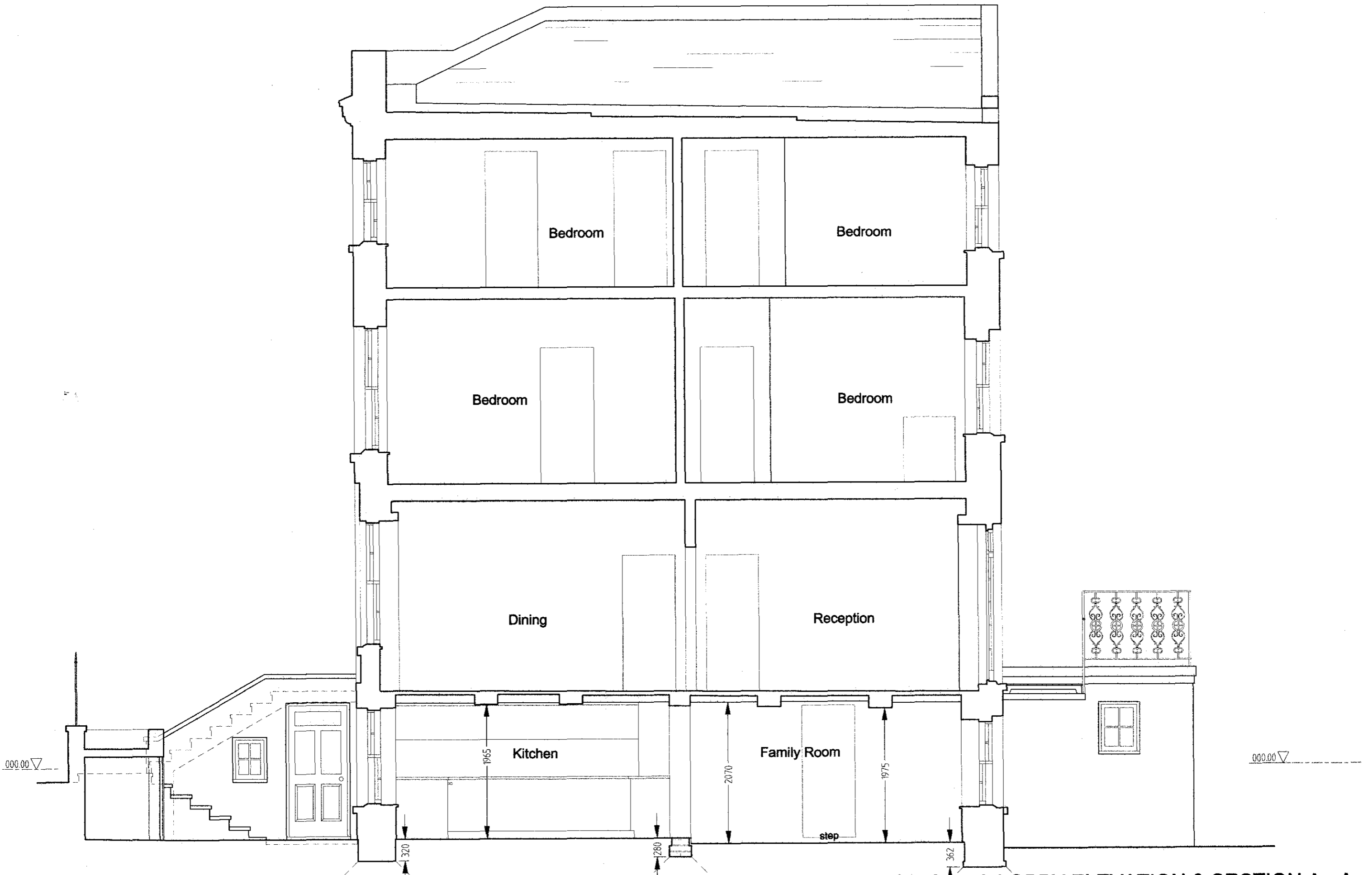
EXISTING LOBBY ELEVATION & SECTION A - A 44 Downshire Hill, London NW3 1NU
