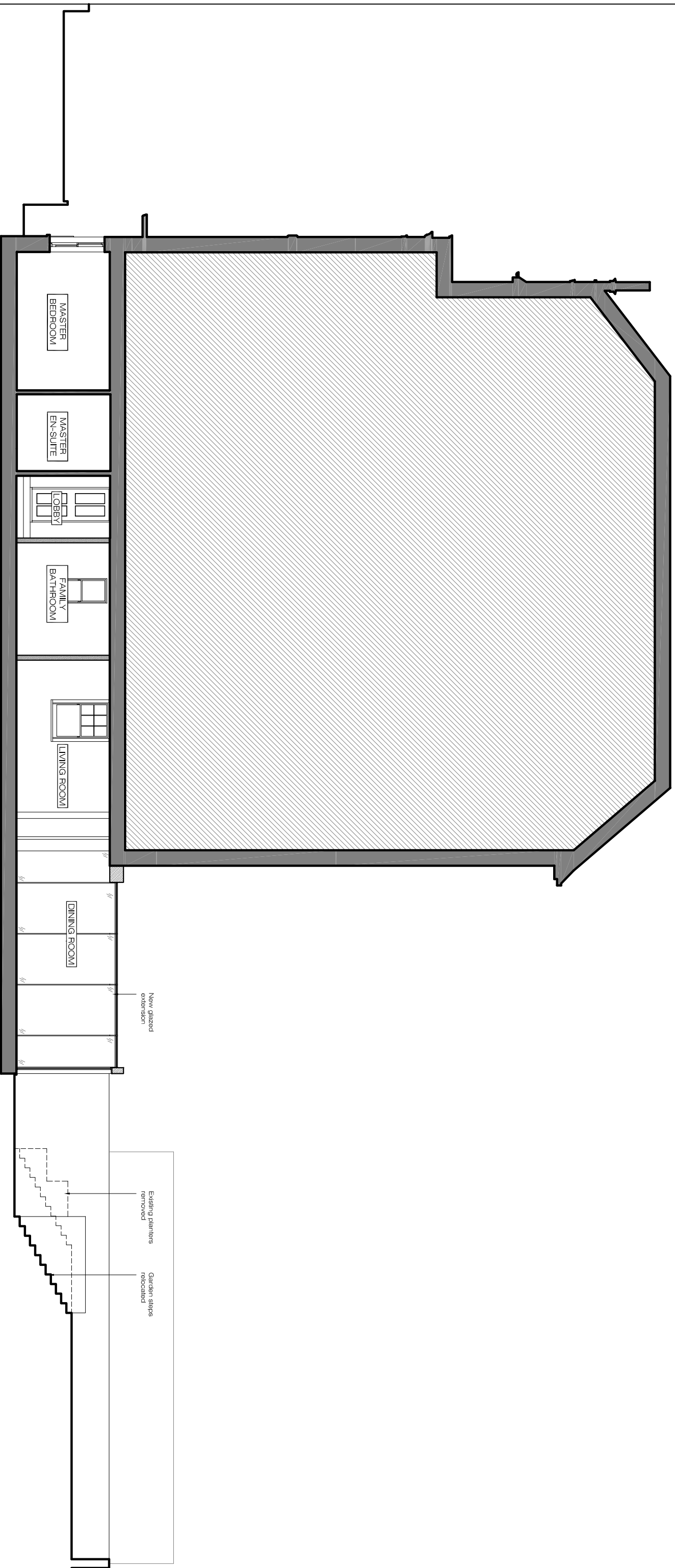
PROPOSED SECTION BB SCALE 1:100@A3 PA-04
