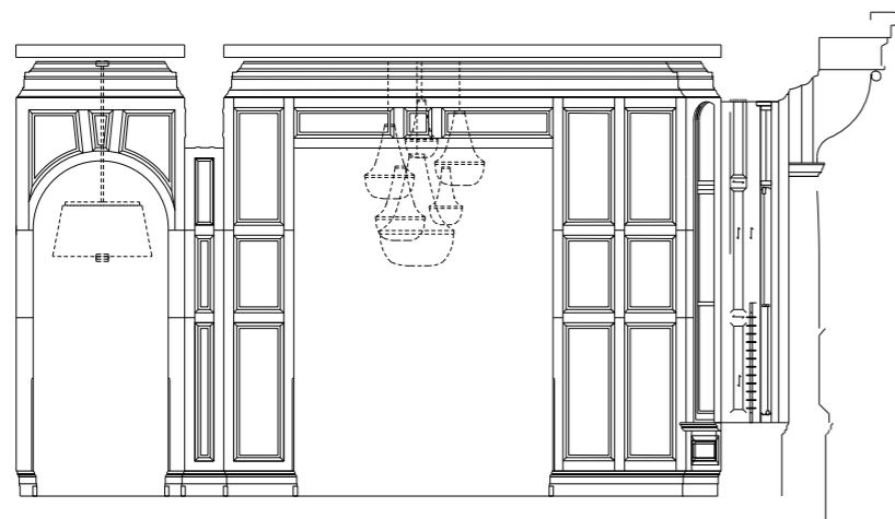
Elevation C
