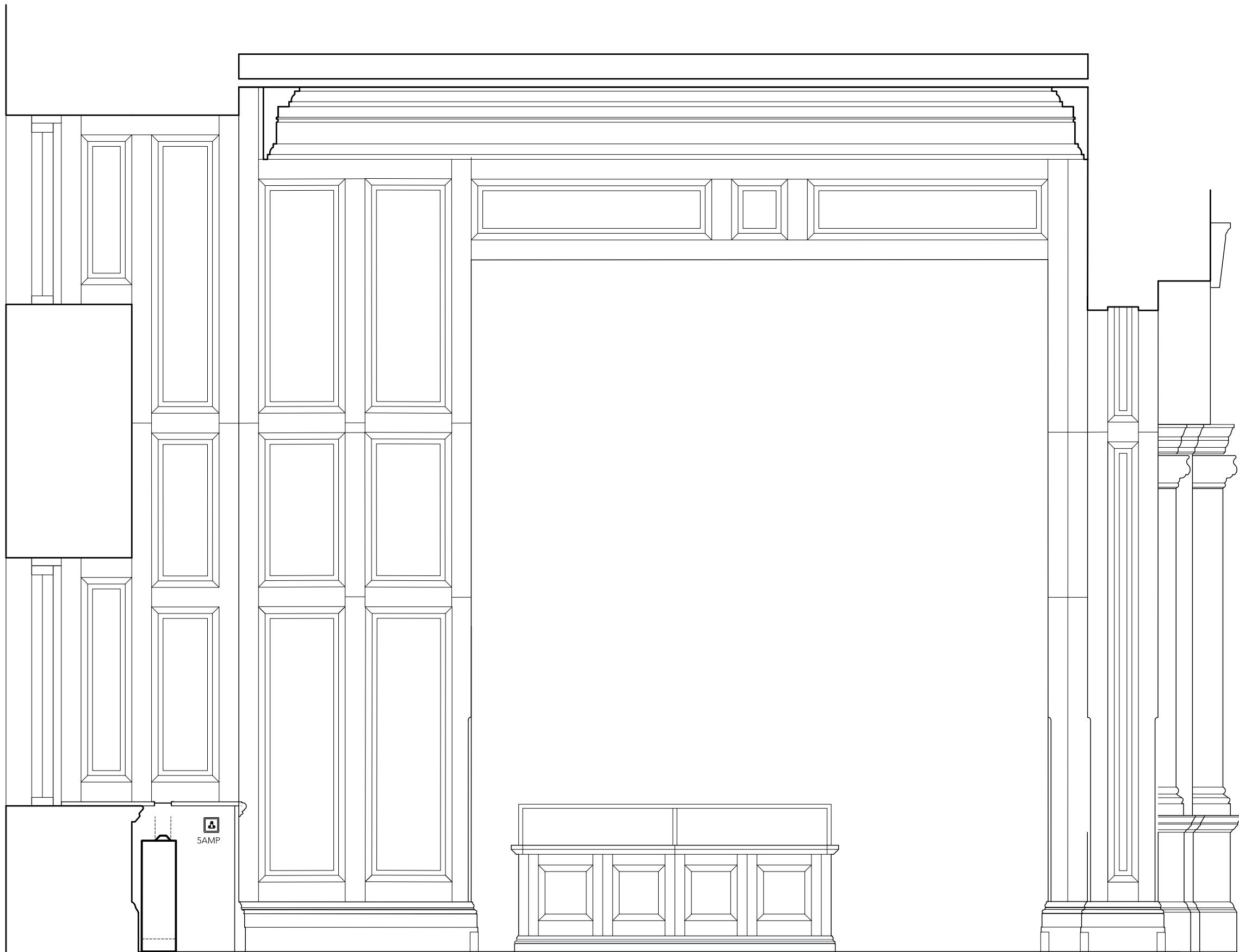
2 ELEVATION D2D scale 1:25
