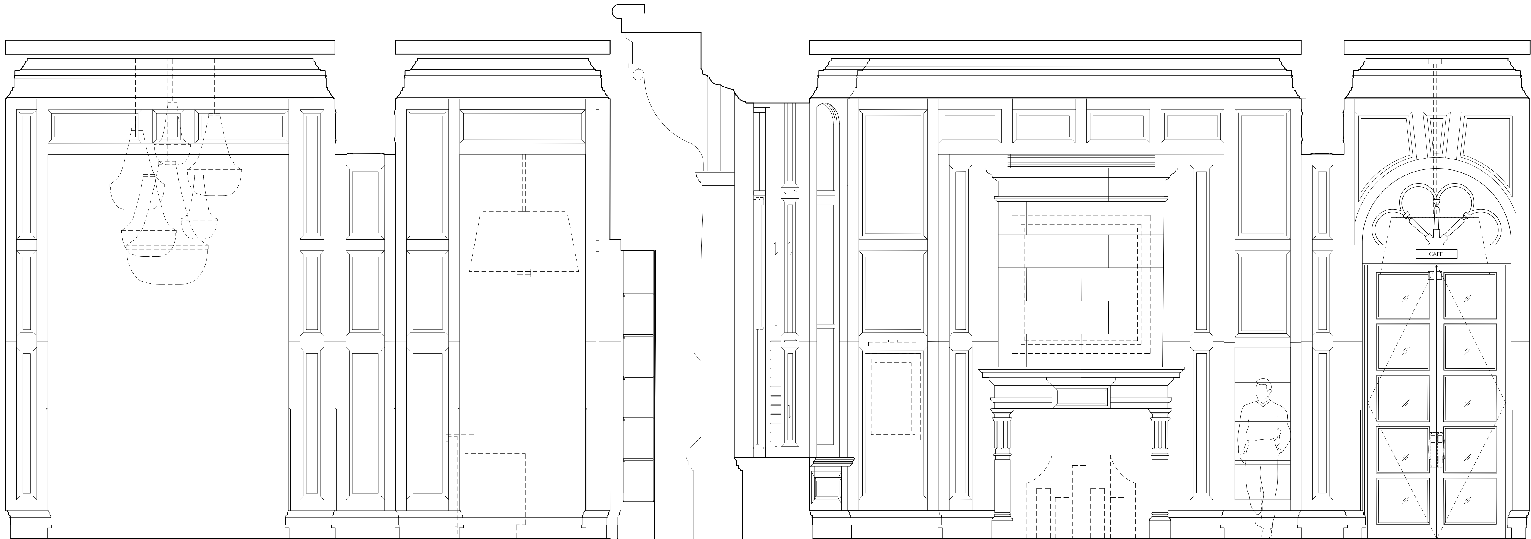
1 ELEVATION D1C scale 1:25
