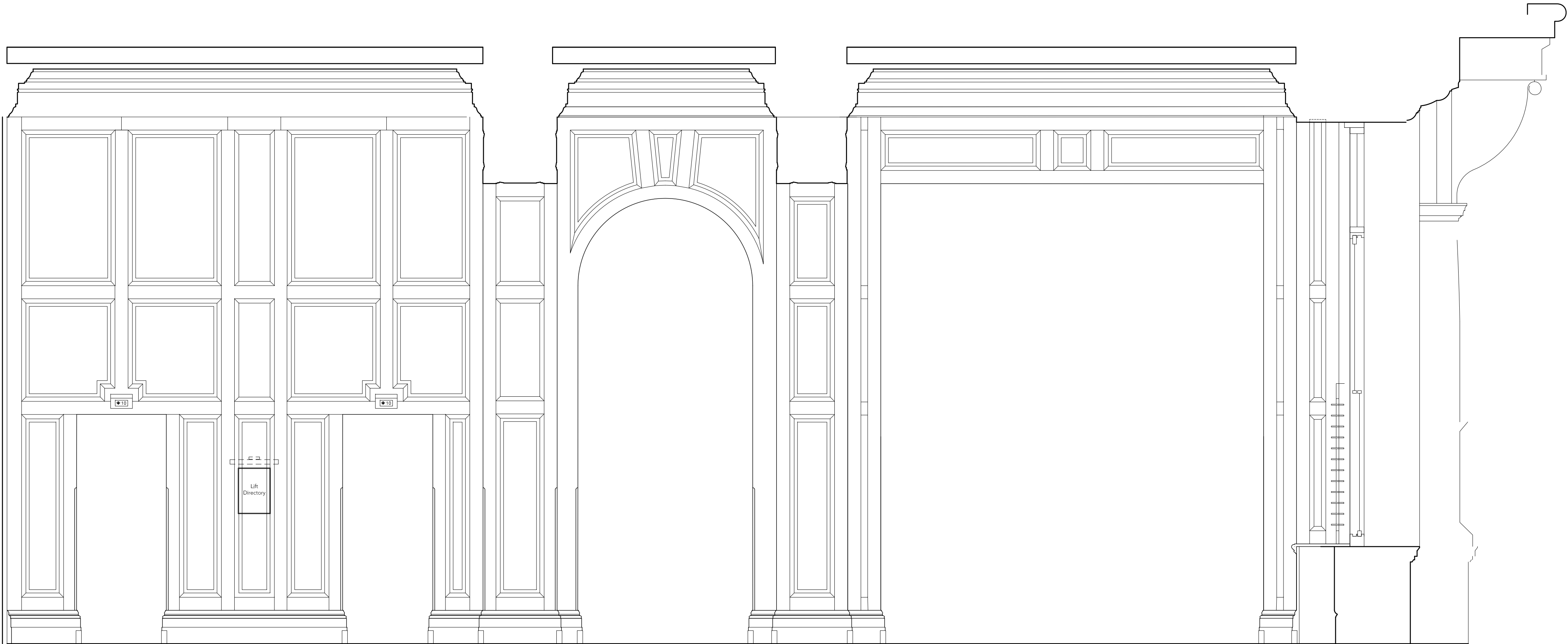
2 ELEVATION D4B scale 1:25
