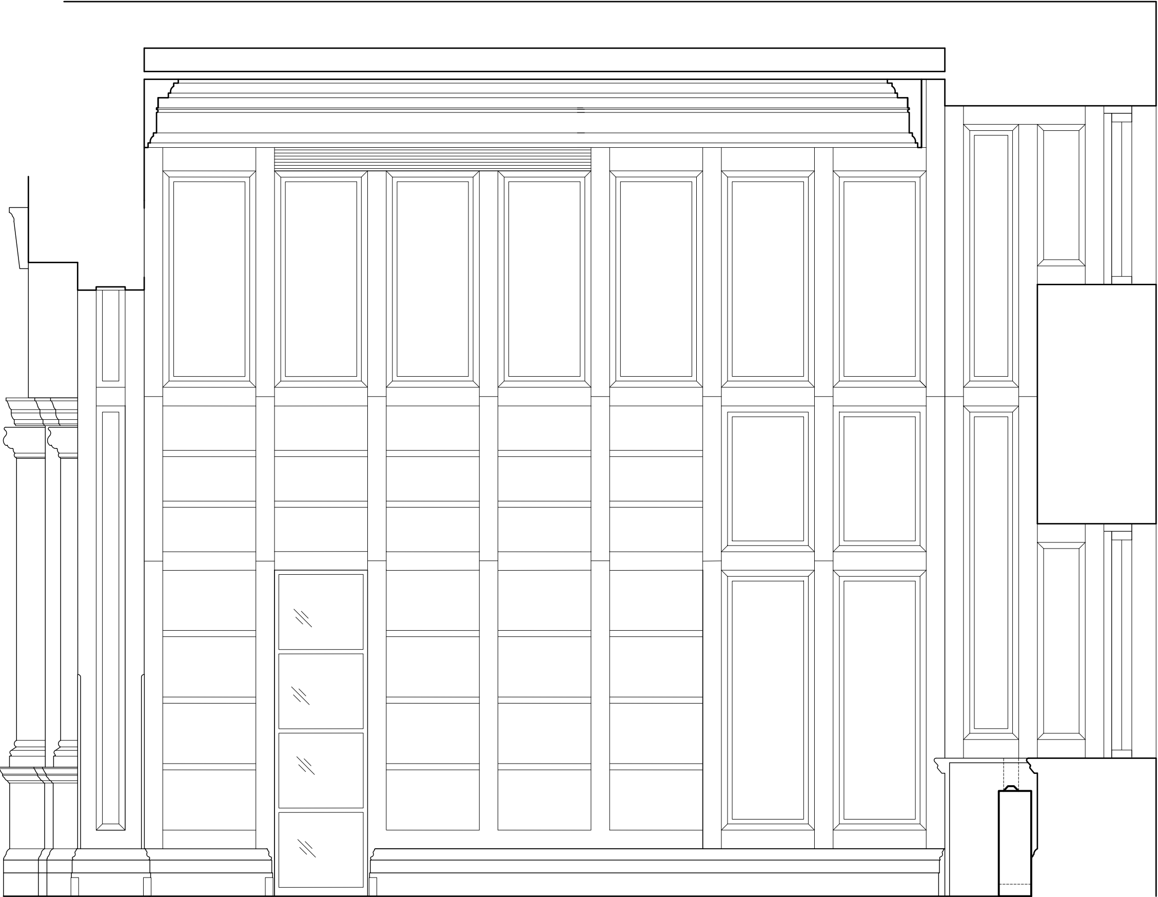
1 ELEVATION D4A scale 1:25
