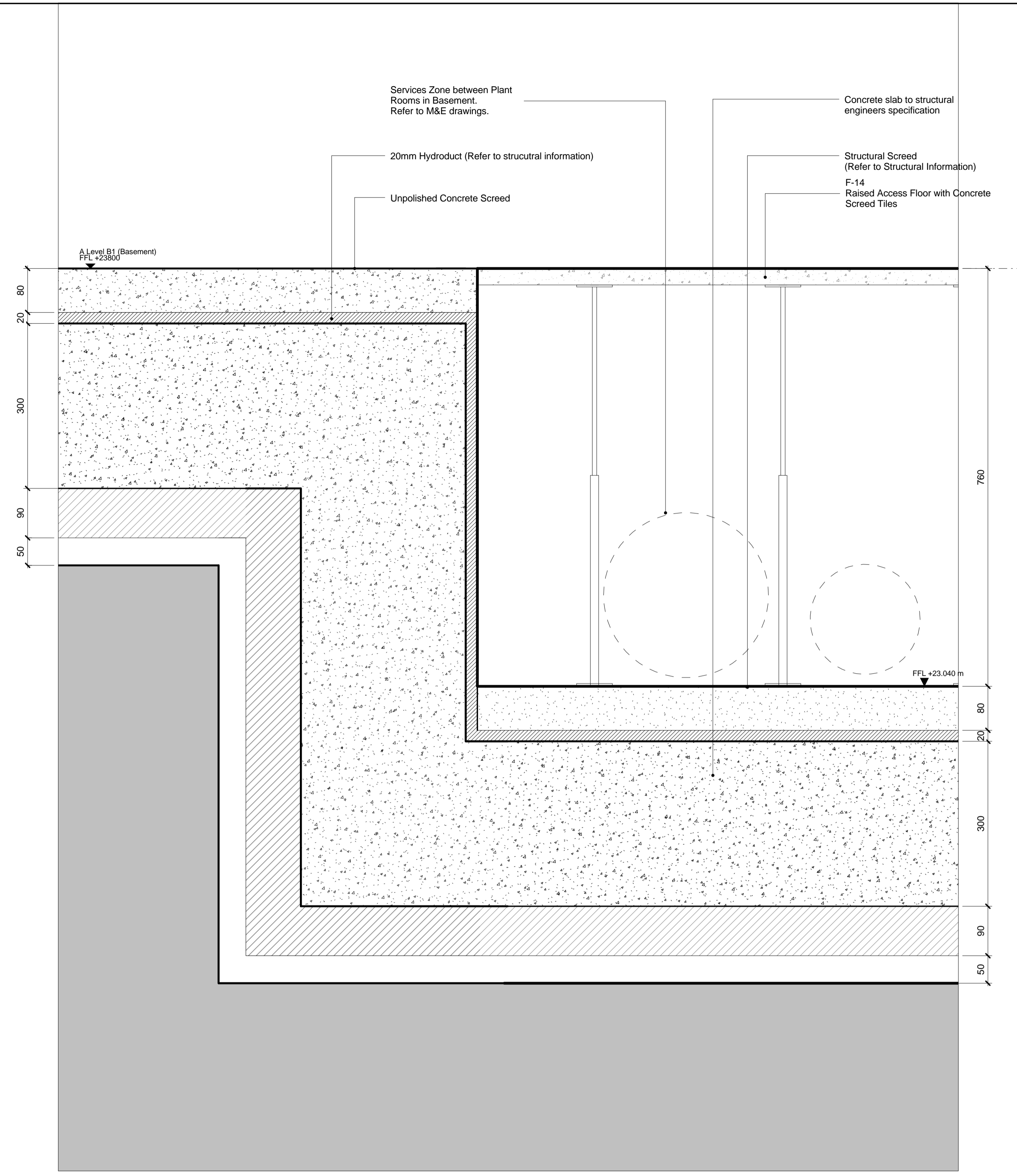
1 Basement Stepped Slab in Corridor
