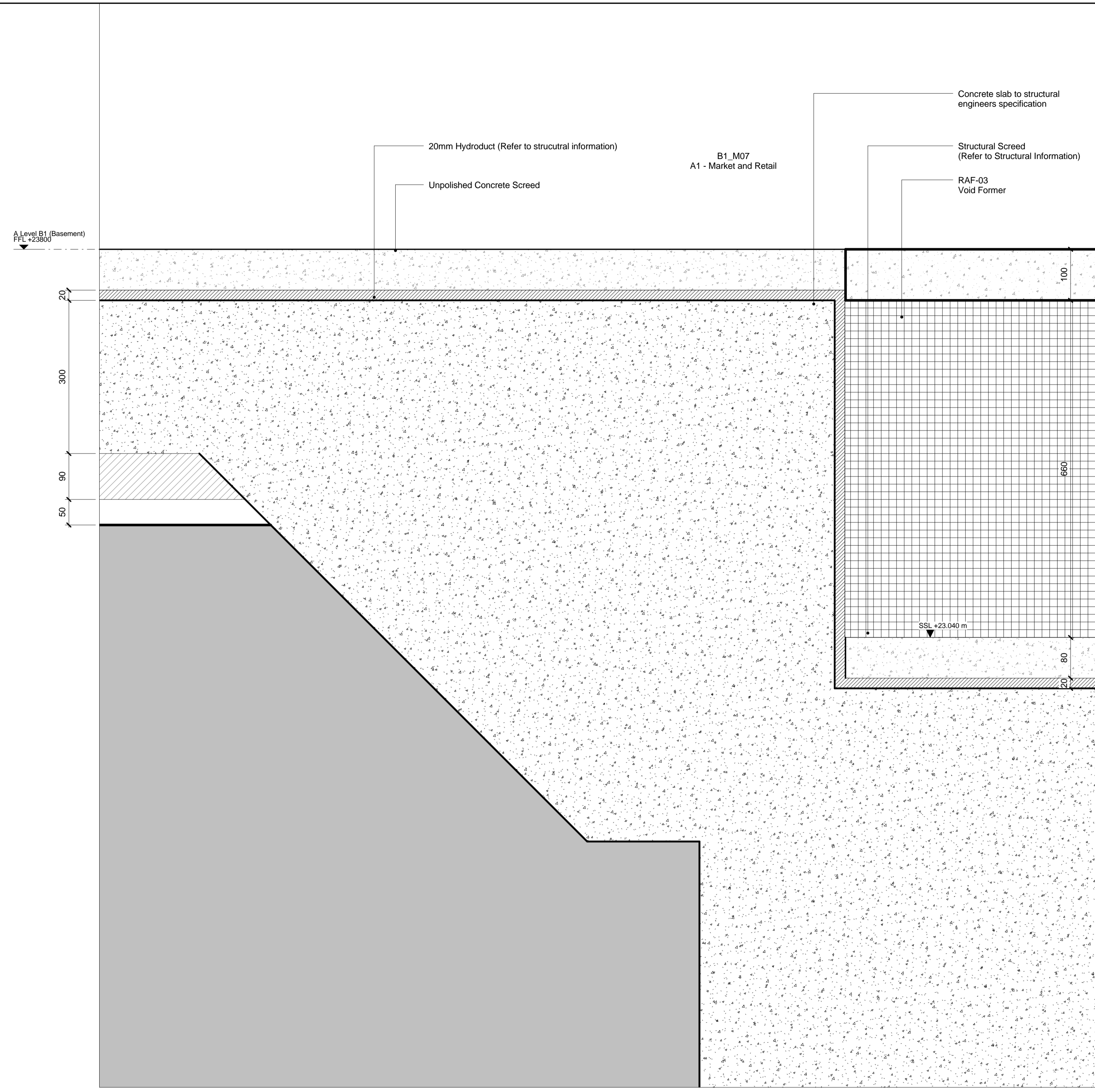
2 Basement Stepped Slab in Market
