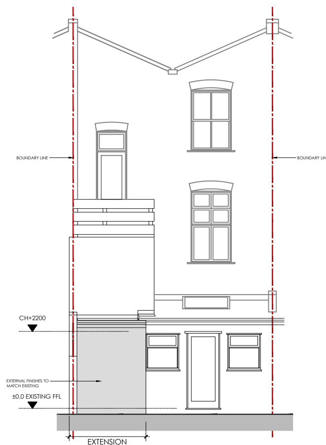
3 ELEVATION-REAR - PROPOSED 1:100
