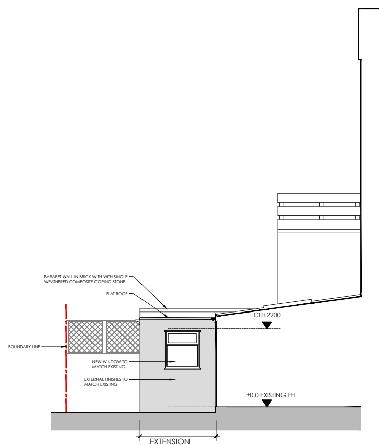
4 ELEVATION-SIDE (SOUTH EAST) - PROPOSED 1:100
