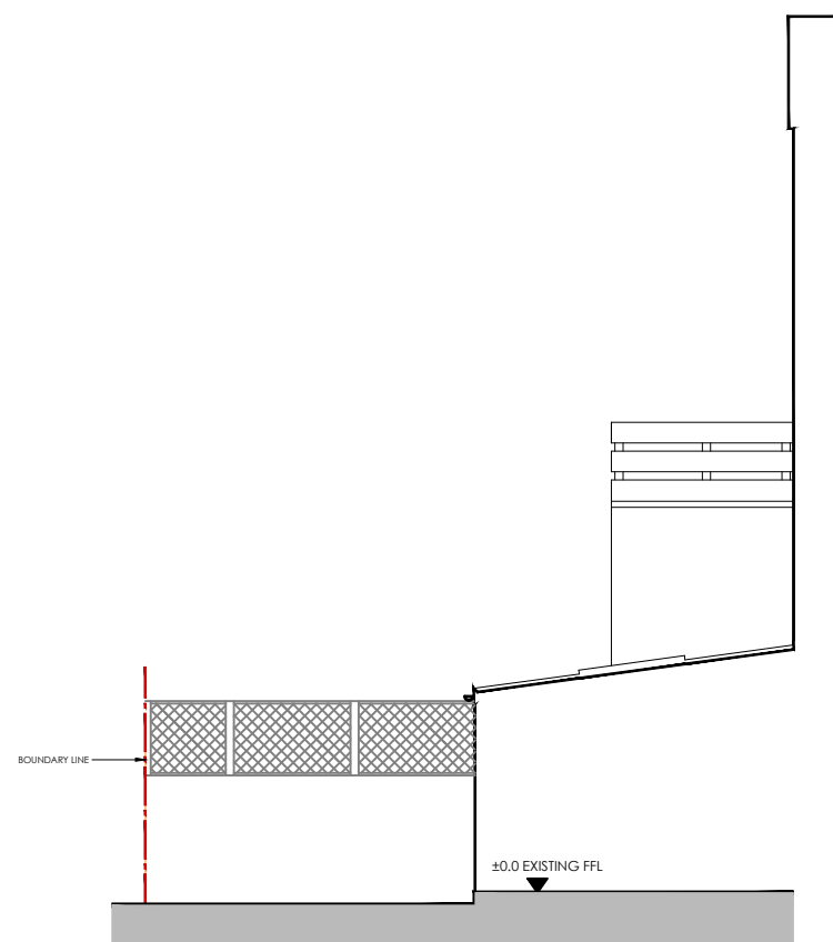
2 ELEVATION-SIDE (SOUTH EAST) - EXISTING 1:100
