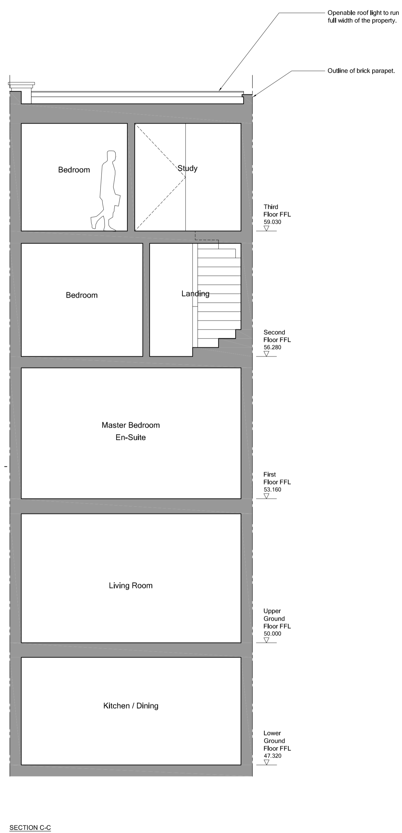
SECTION C-C
