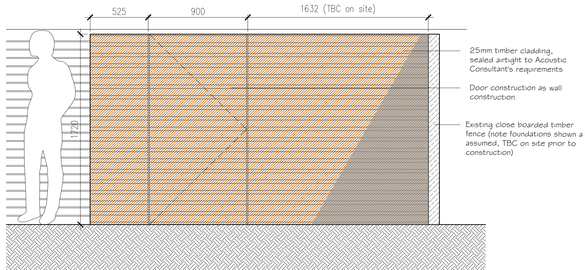
Proposed Enclosure for Plant Equipment Section B-B
