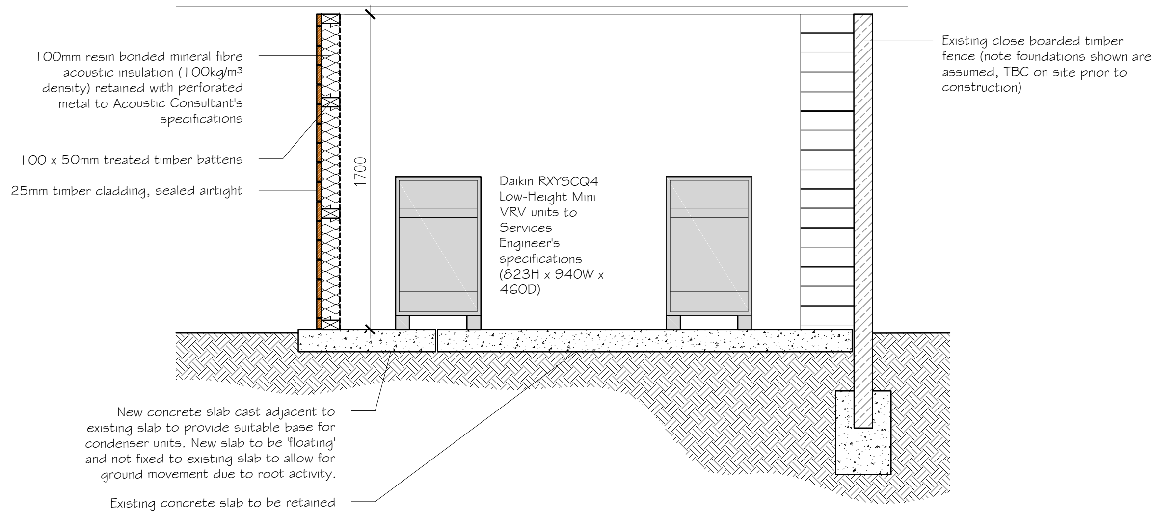
Proposed Enclosure for Plant Equipment Section D-D
