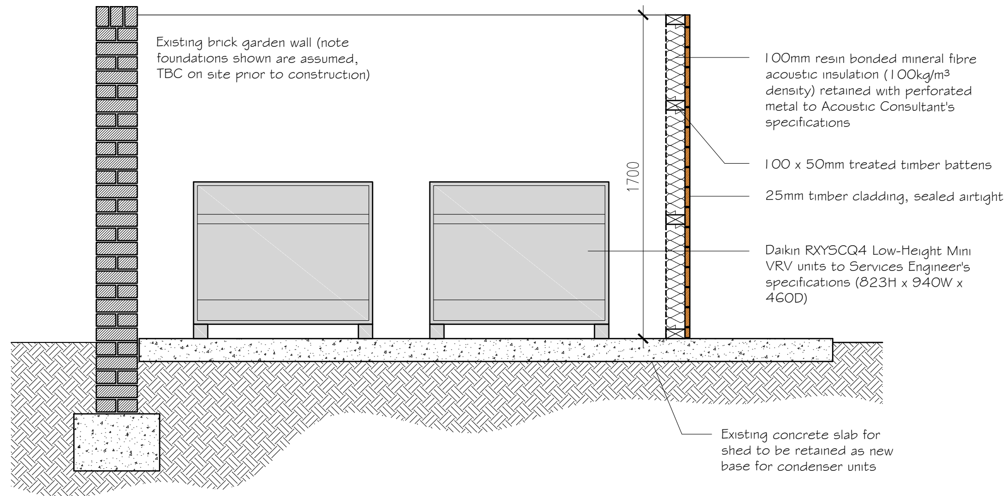
Proposed Enclosure for Plant Equipment Section C-C
