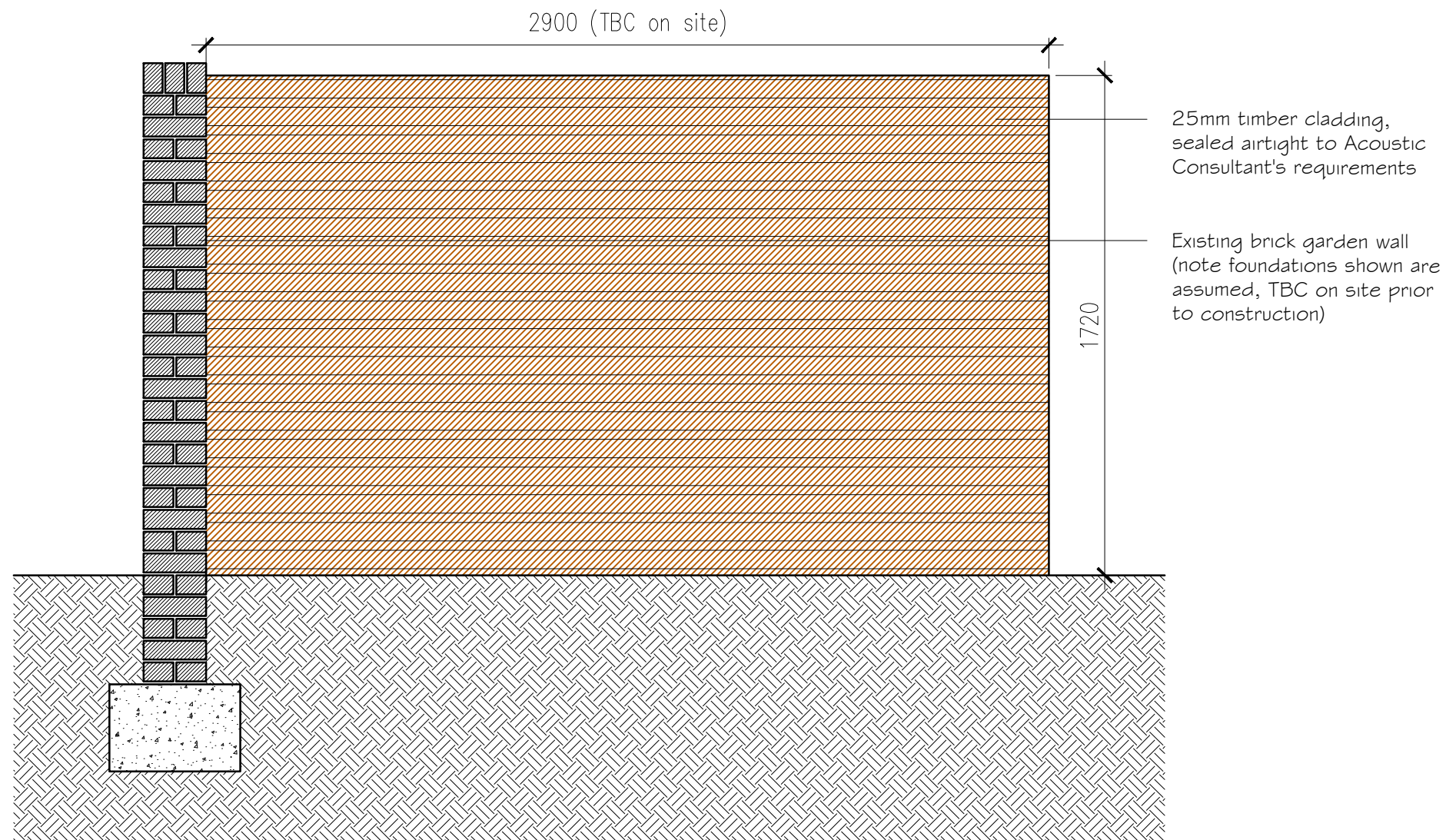
Proposed Enclosure for Plant Equipment Section A-A
