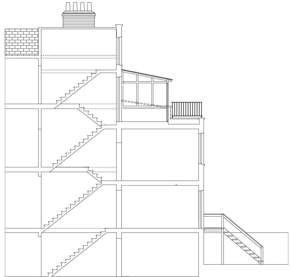
PART SECTION A-A
