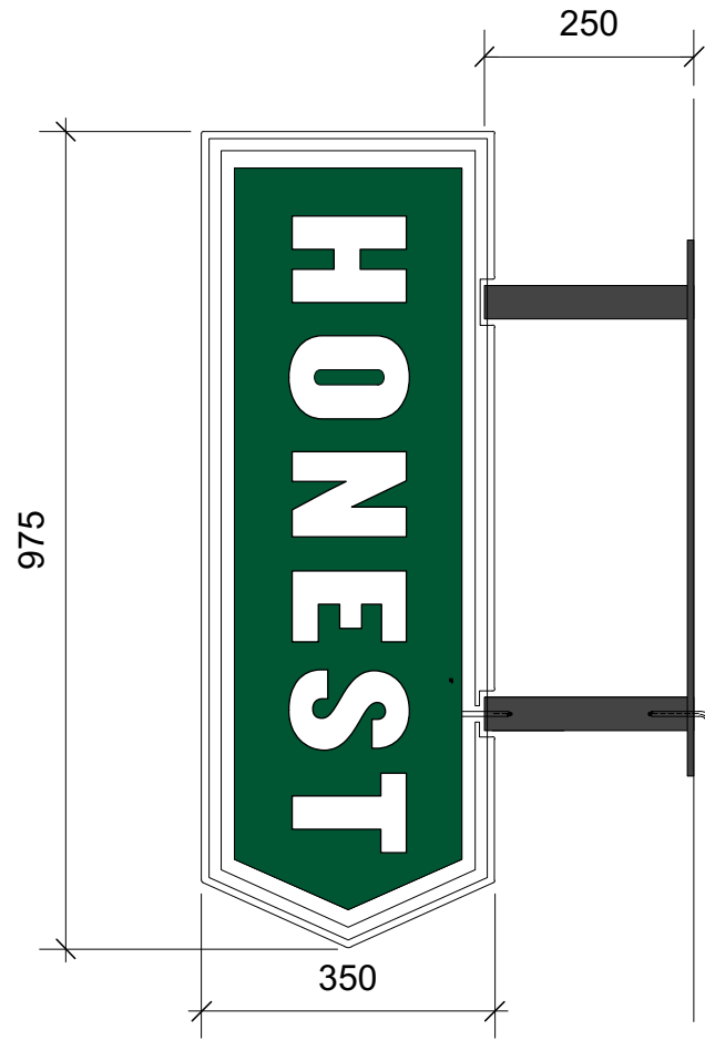
FRONT ELEVATION 1:10@A3
