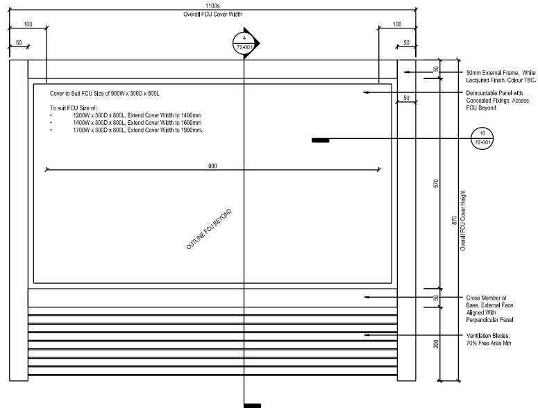
5 | FCU Housing - Front Elevation 1:5
