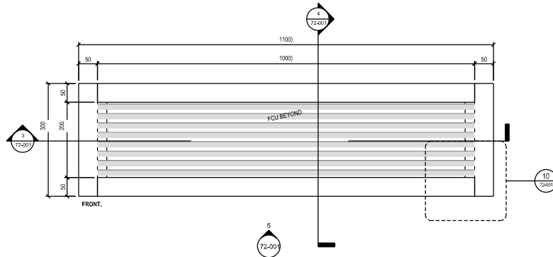
2 | FCU Housing - Plan Detail 1:5
