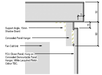
10 | Detail - Panel Fixing 1:2
