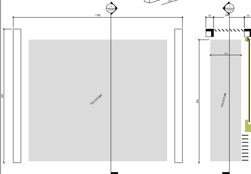
3 | FCU Housing - Section Detail AA 1:5
