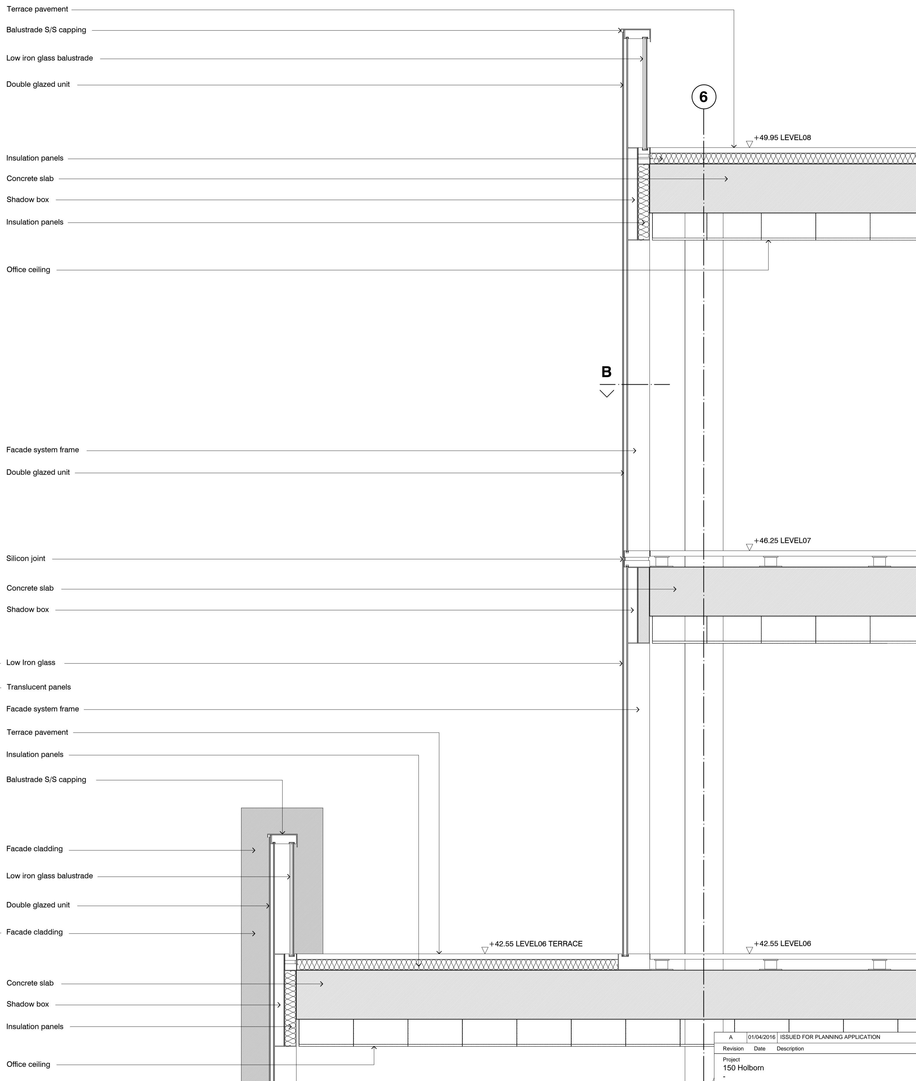
Section A
