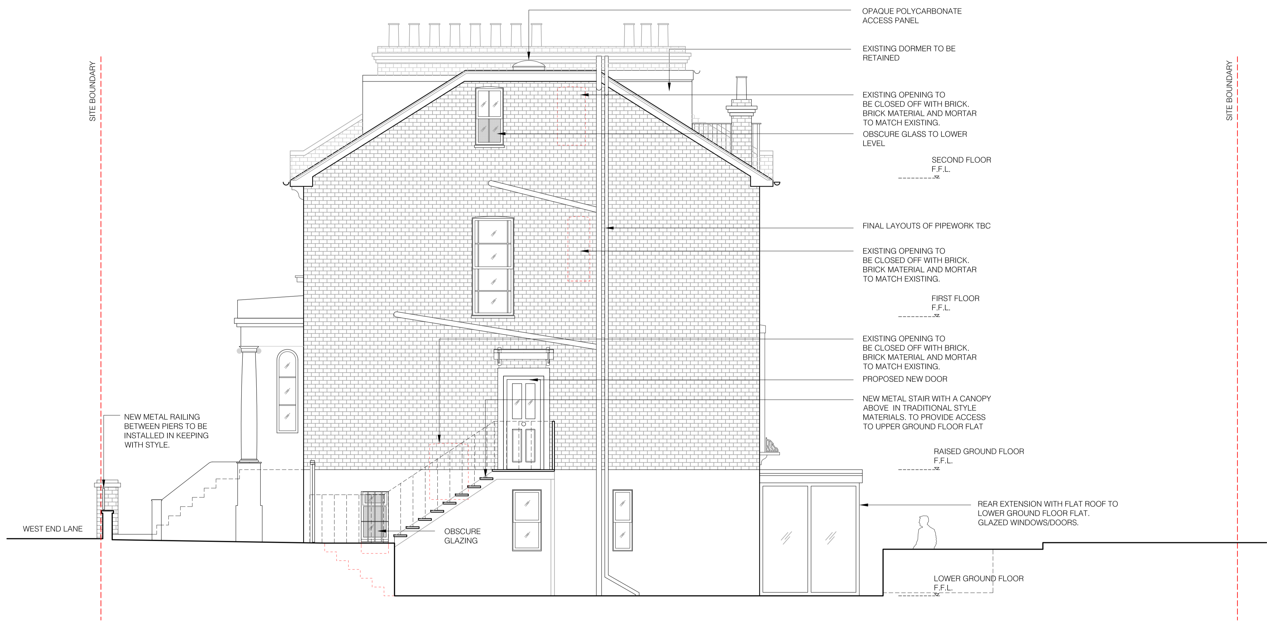
1 PROPOSED SIDE ELEVATION
