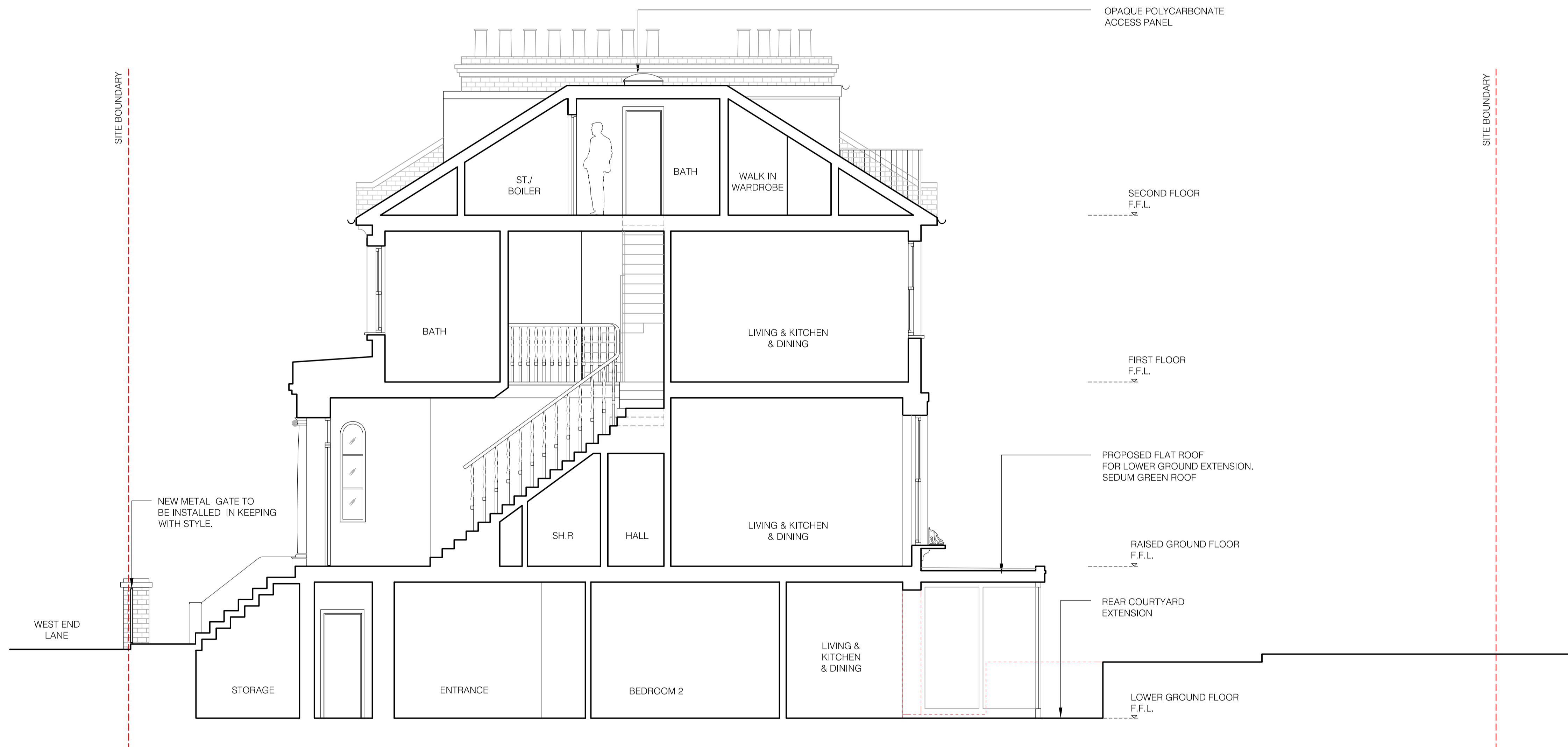
1 PROPOSED SECTION
