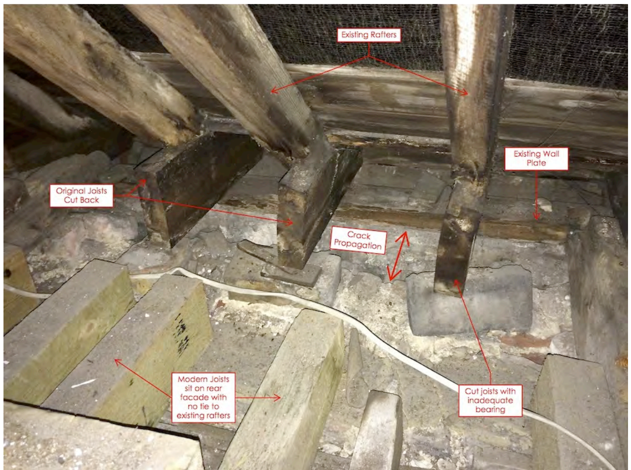
Rear eaves void (annotations by structural engineer)
