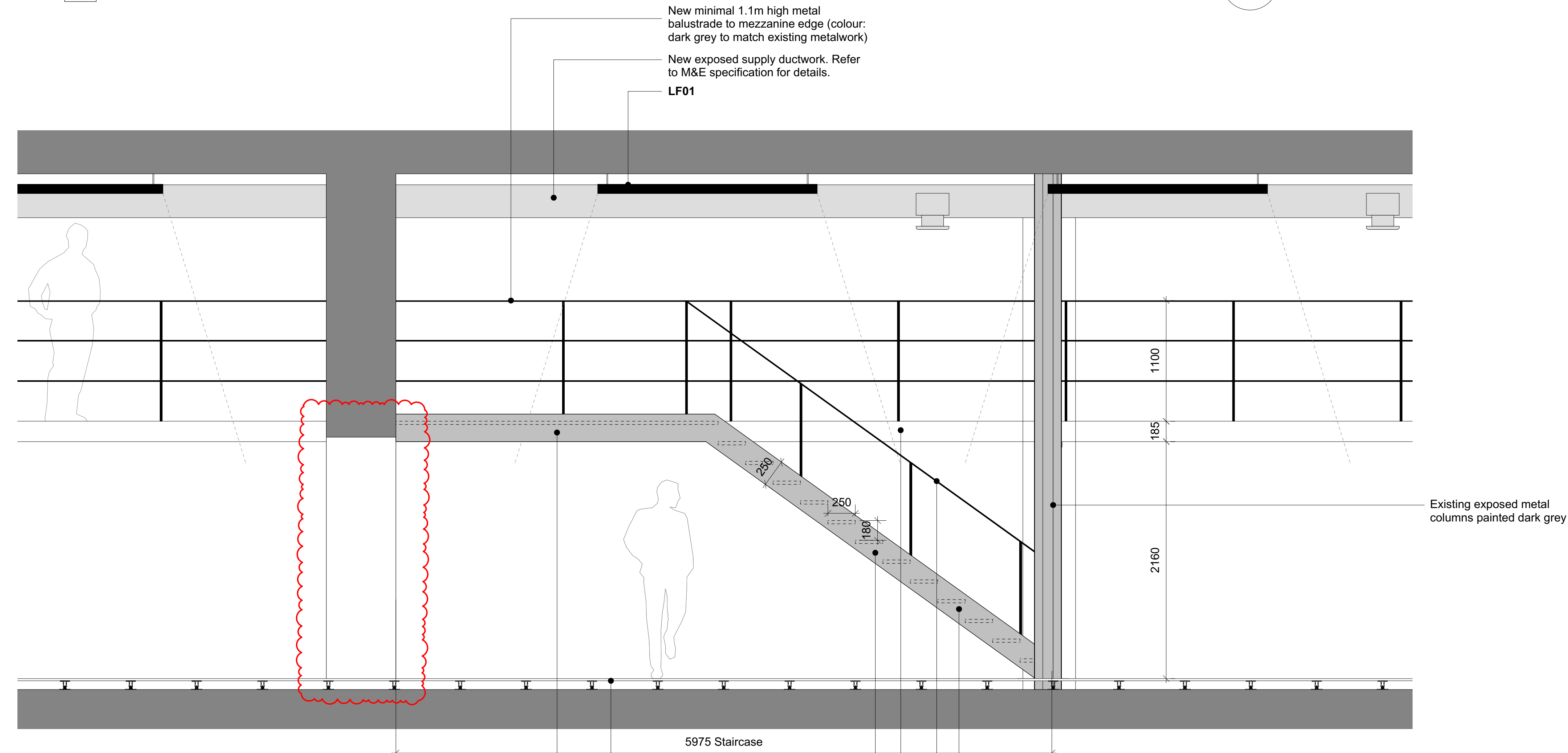
1 Proposed Section BB (203 Eversholt St) Scale 1:50 @ A1 / 1:100 @ A3
