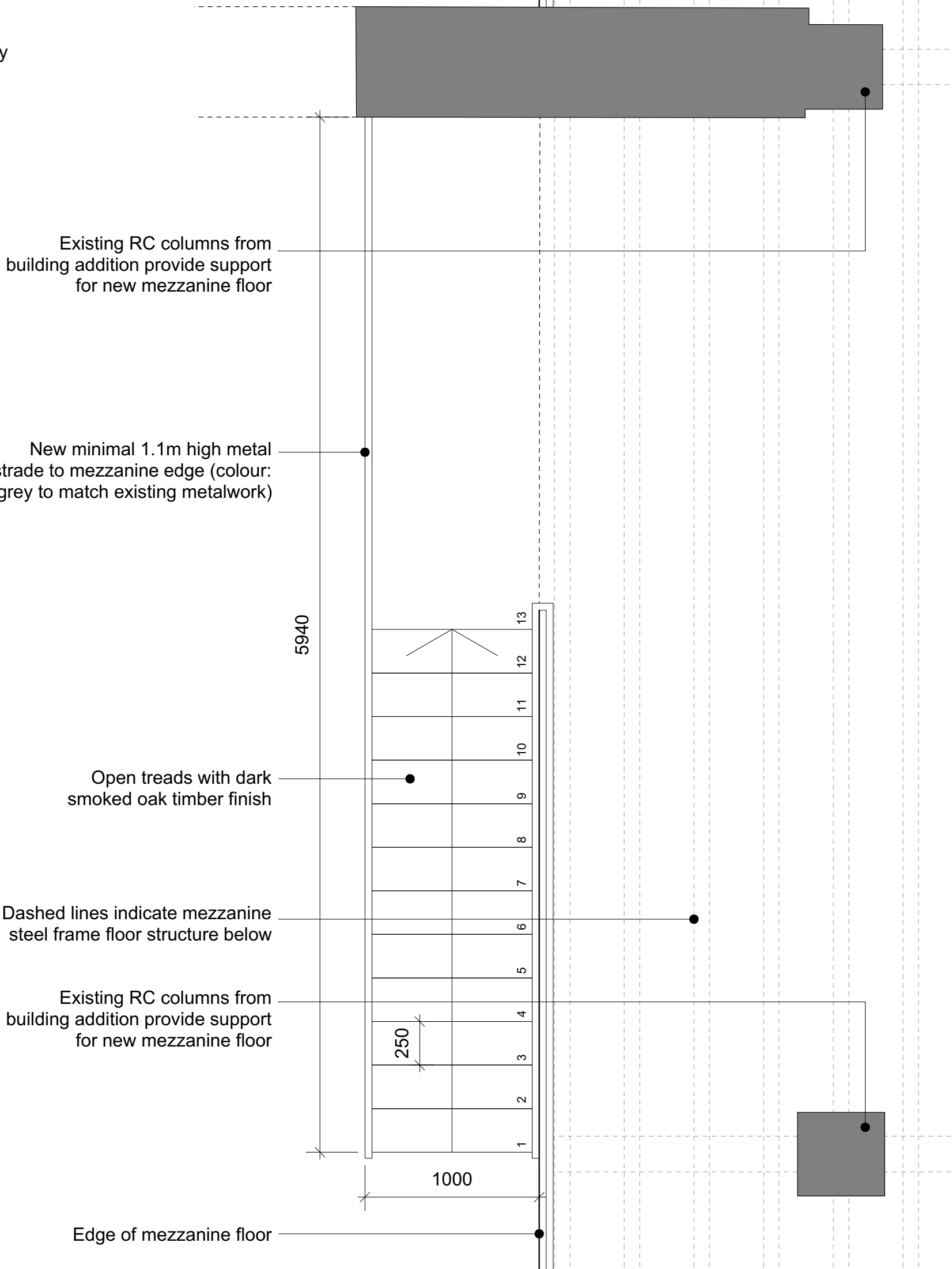
3 Proposed Detailed Stair Plan (203 Eversholt St) Scale 1:25 @ A1 / 1:50 @ A3
