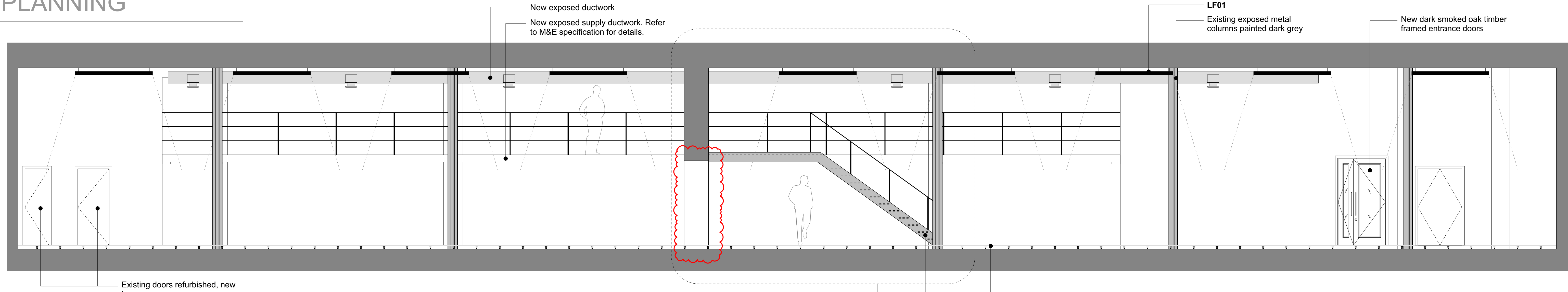
1 Proposed Section BB (203 Eversholt St) Scale 1:50 @ A1 / 1:100 @ A3
