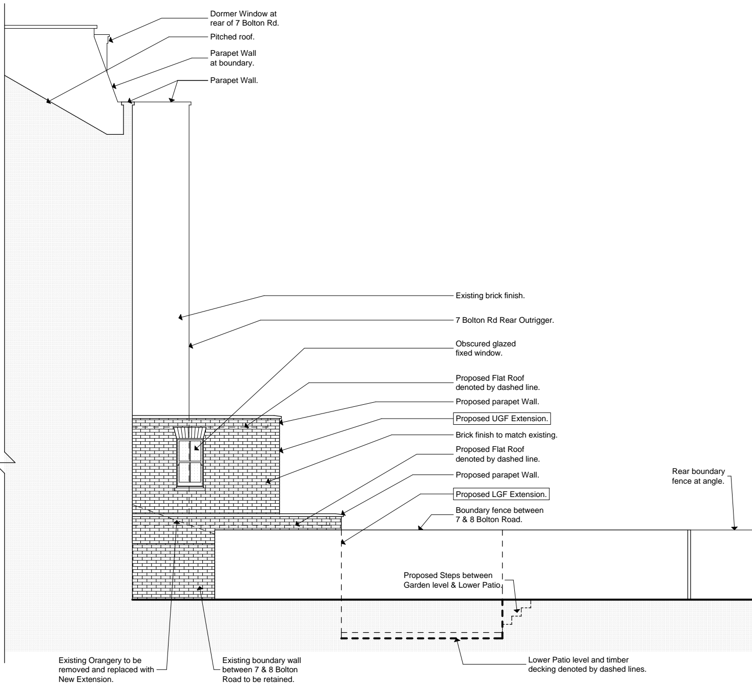
Proposed West Elevation (taken through 8 Bolton Rd)
