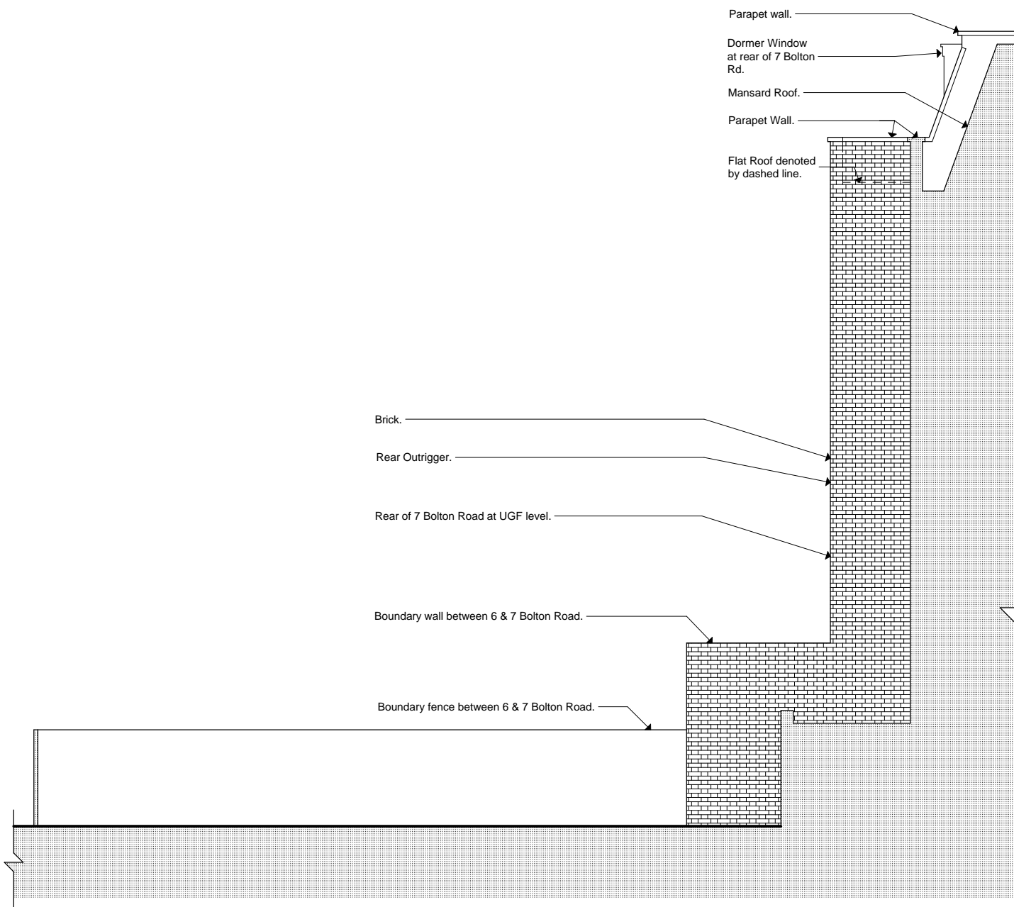
Existing East Elevation (taken through 6 Bolton Rd)
