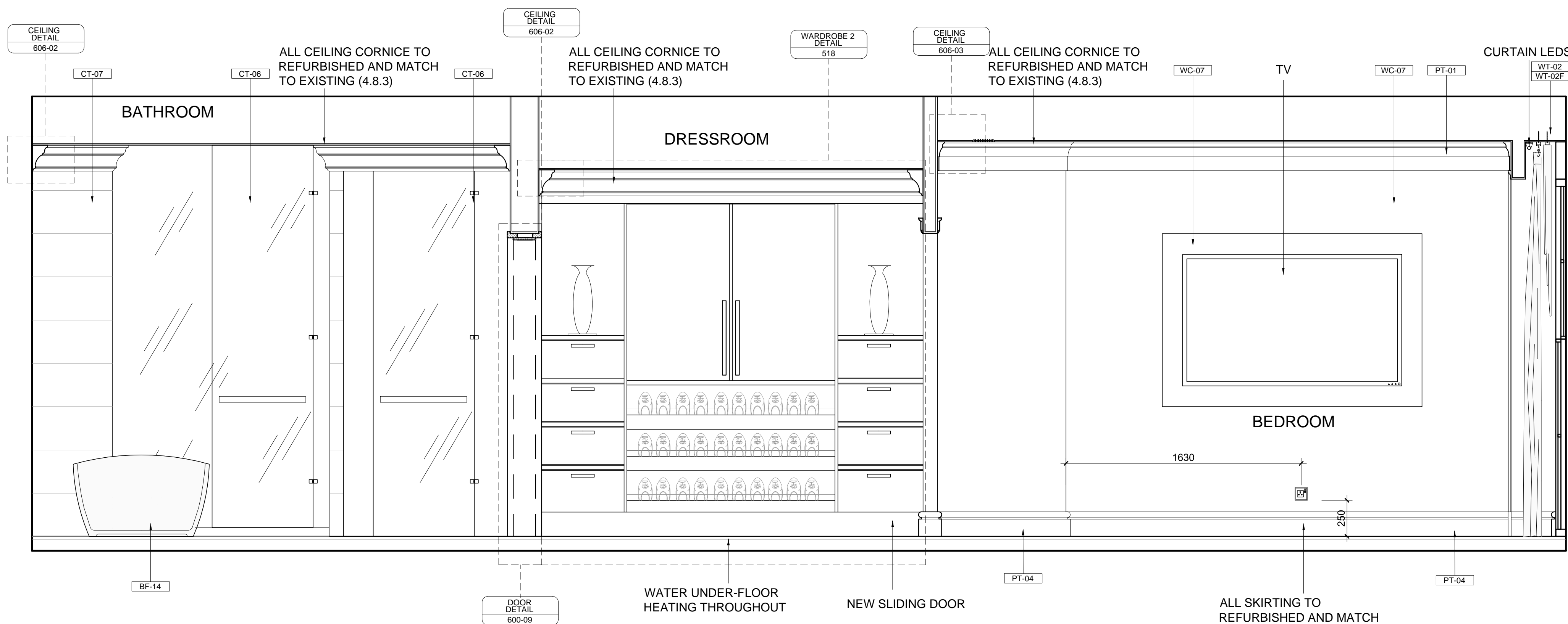
ELEVATION F
