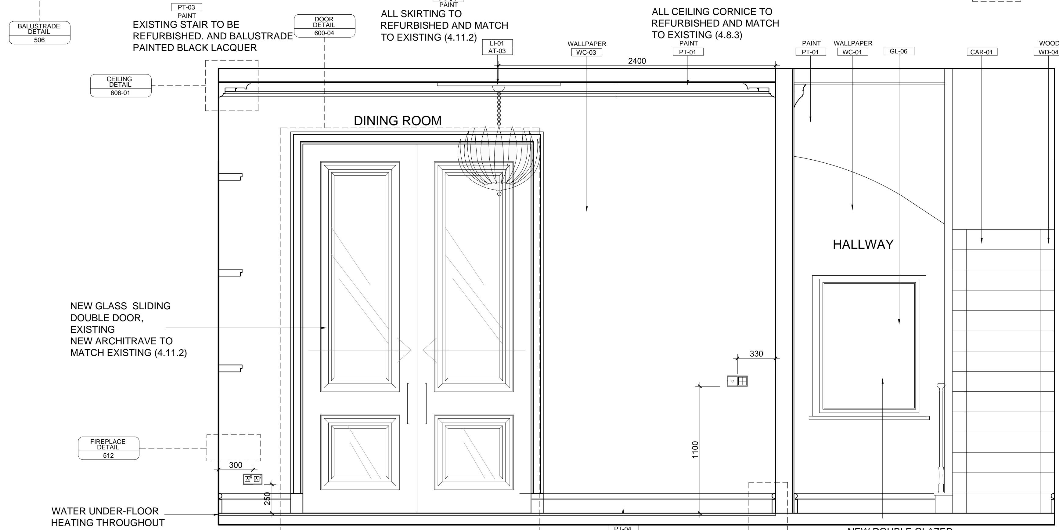
ELEVATION H
