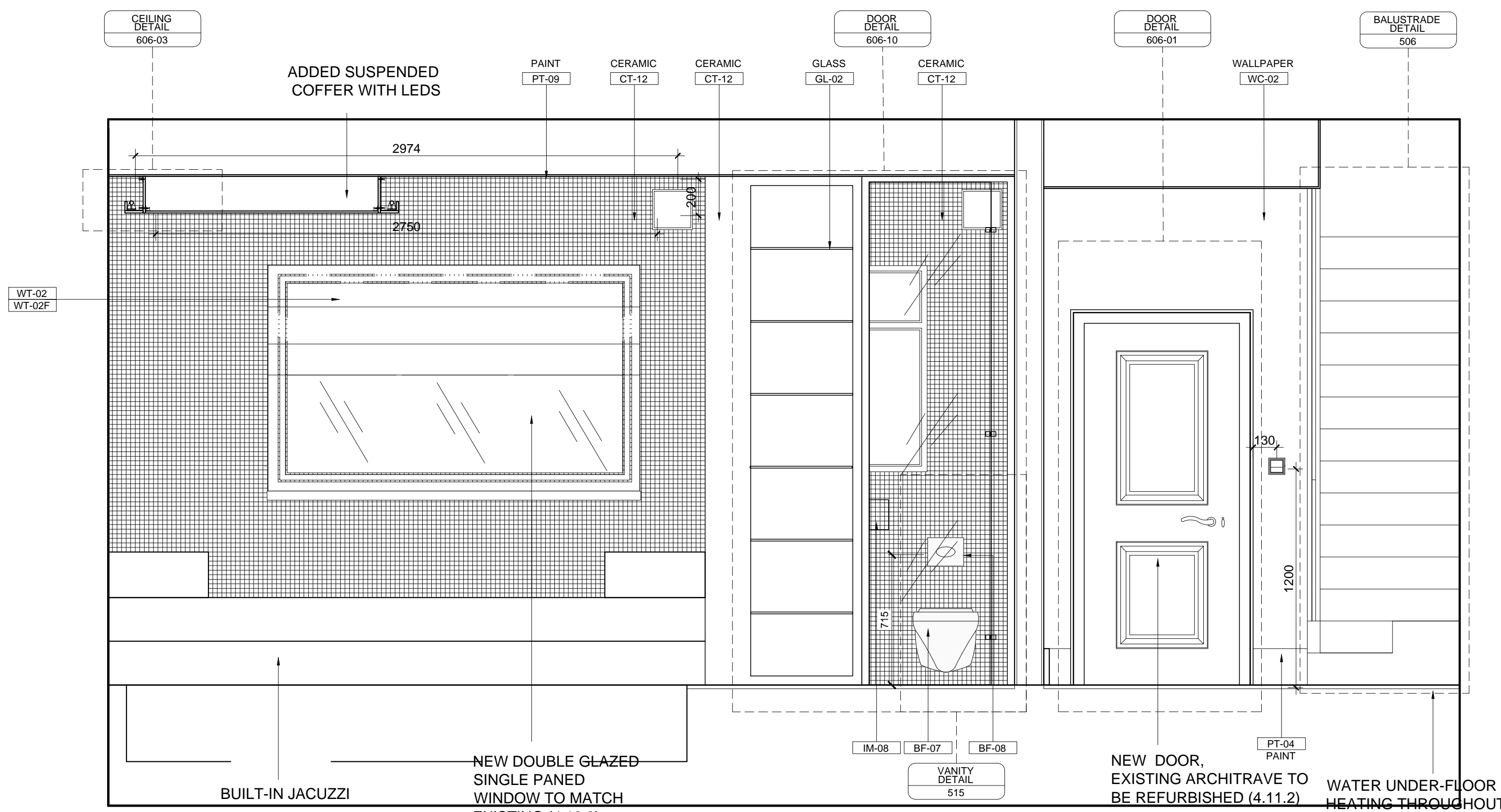
ELEVATION F
