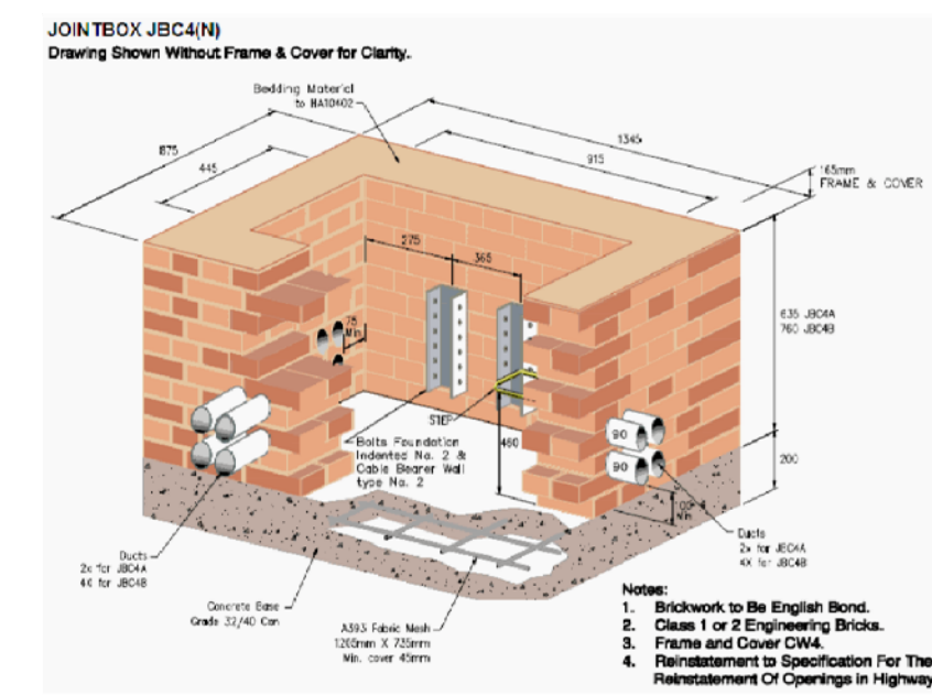
B DETAIL BT DEVELOPERS GUIDE TYPICAL JOINTING CHAMBER CONSTRUCTION NTS
