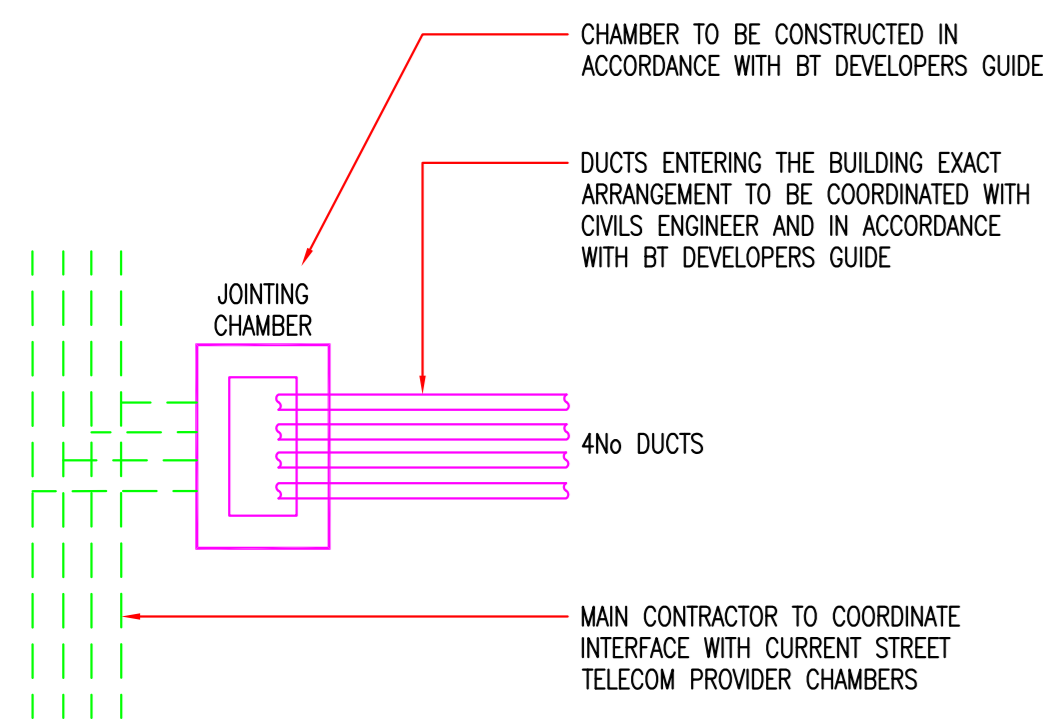
A DETAIL JOINTING CHAMBER DETAIL NTS
