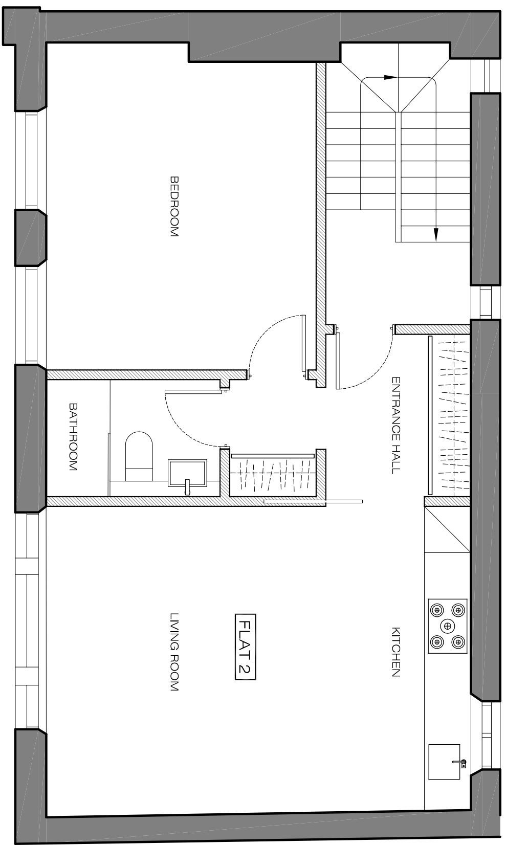
PROPOSED First Floor Plan SCALE 1:50@A3 PA-02
