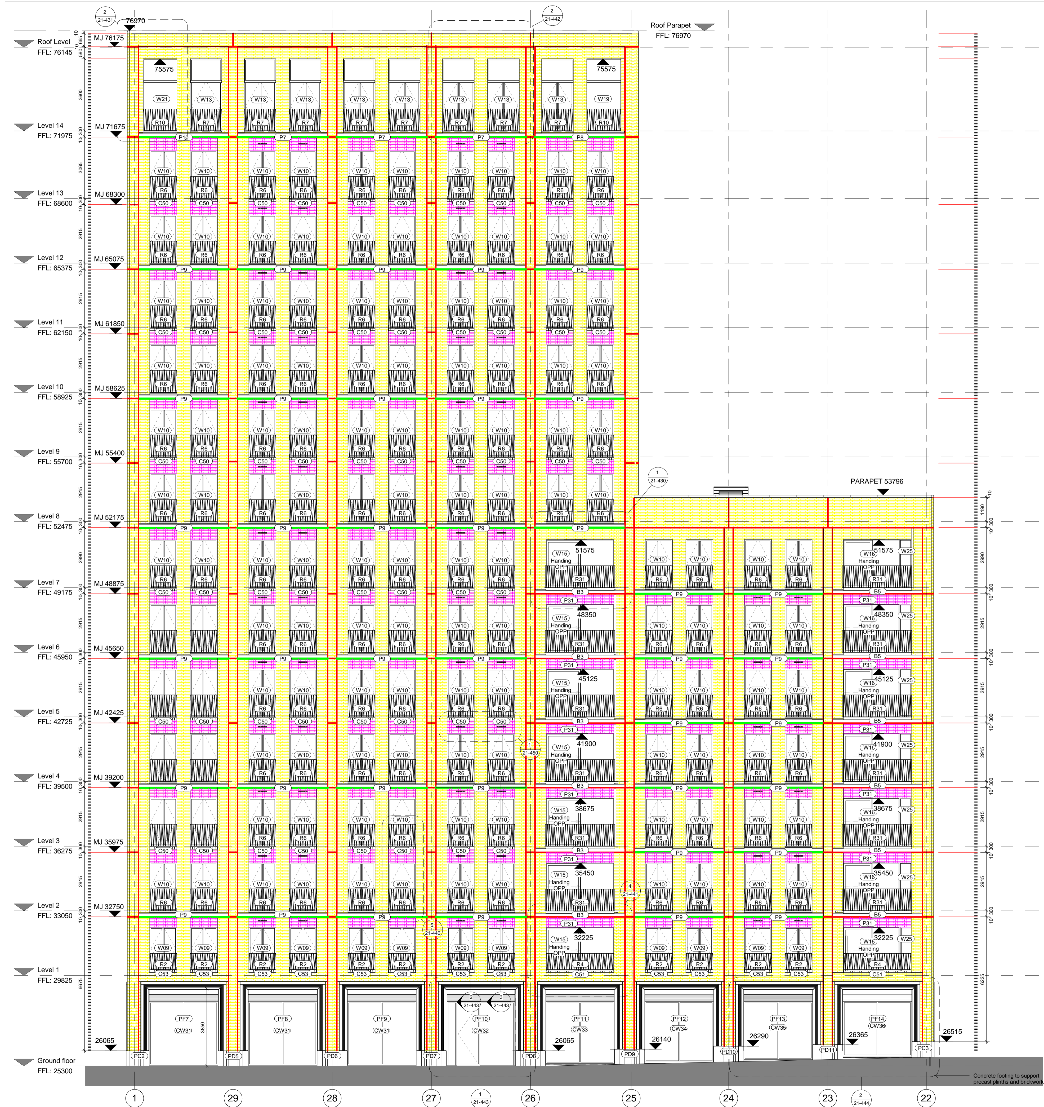
Scoping Elevation South 1:100
