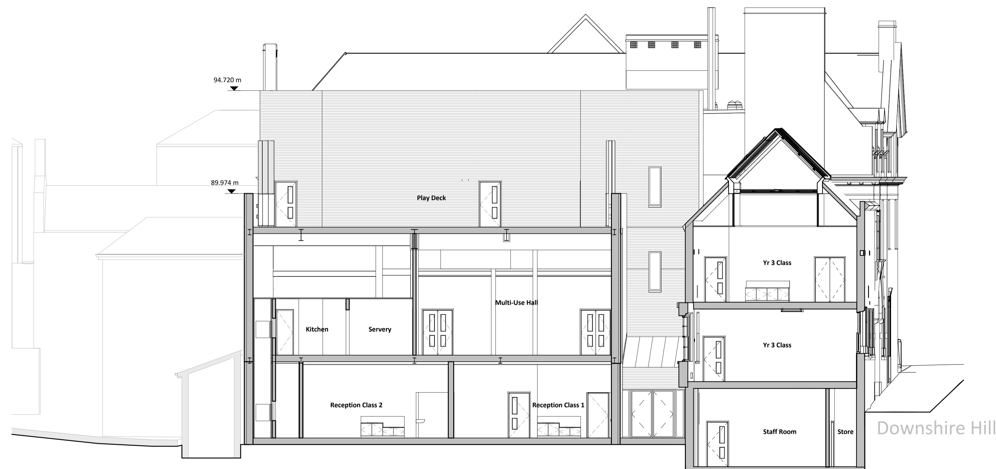
Proposed Section B 1 : 100
