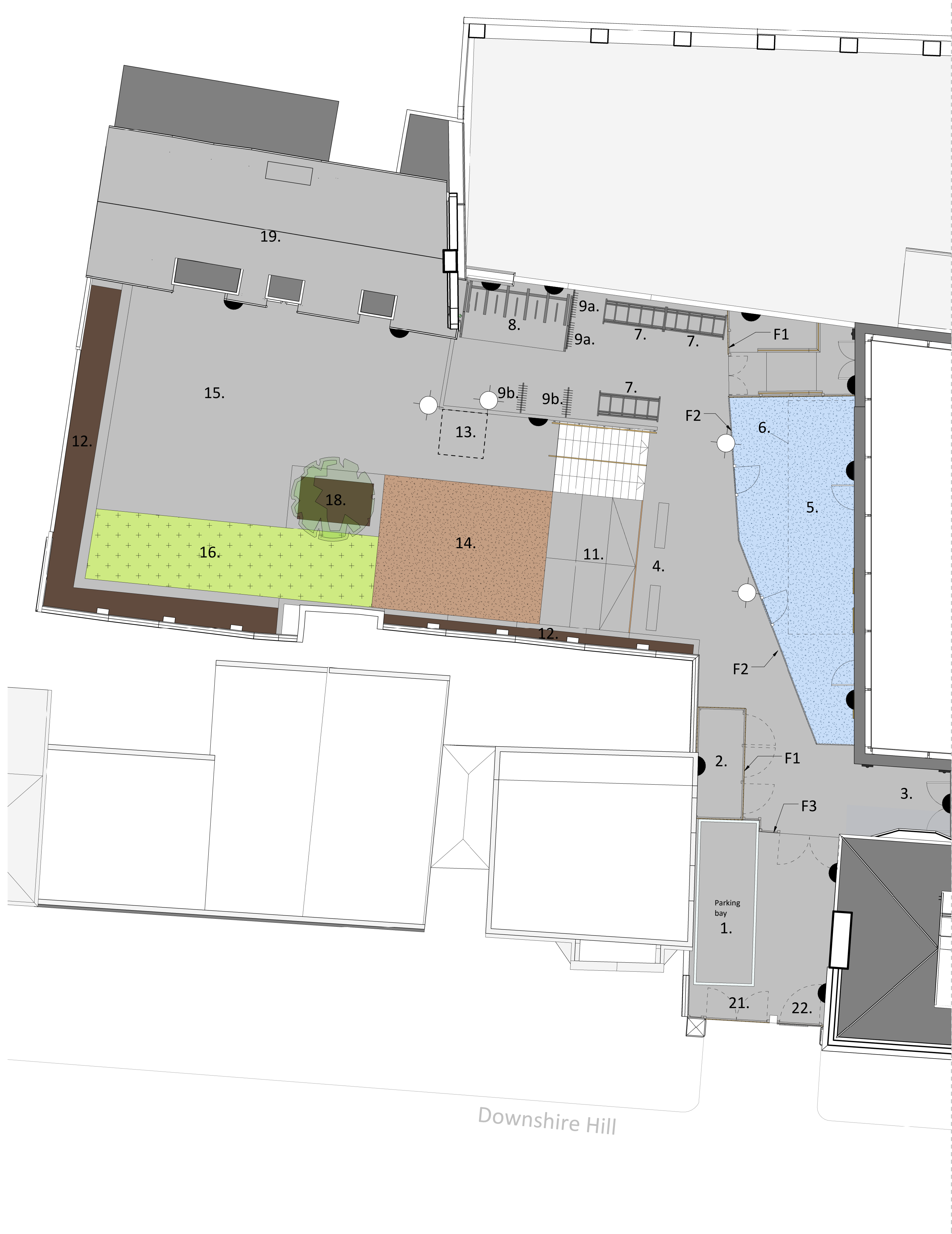
Proposed Landscape Plan 1 : 100
