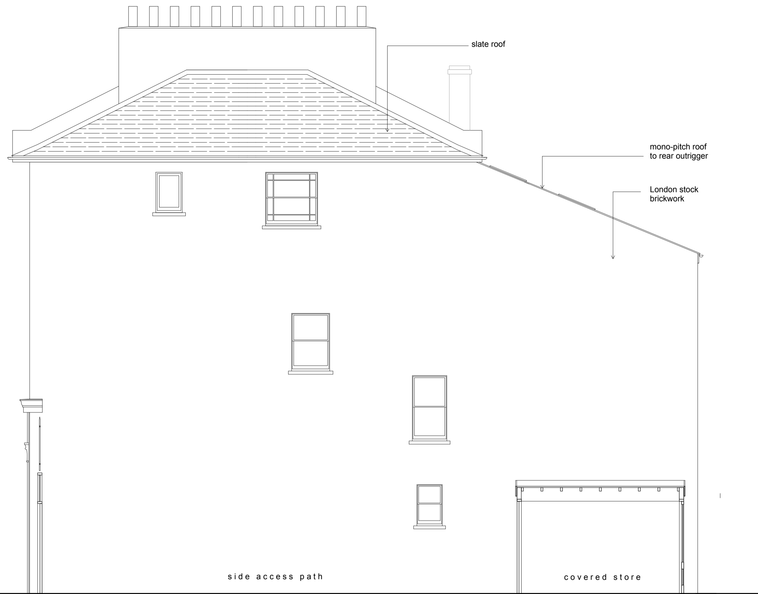
SIDE ELEVATION
