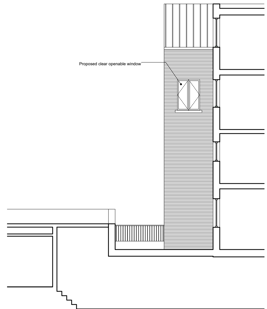
PR WINDOW AT 3FL ELEVATION C
