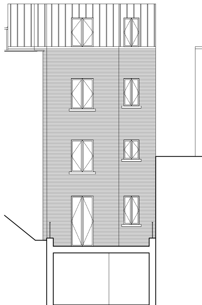
PR WINDOW AT 3FL ELEVATION B
