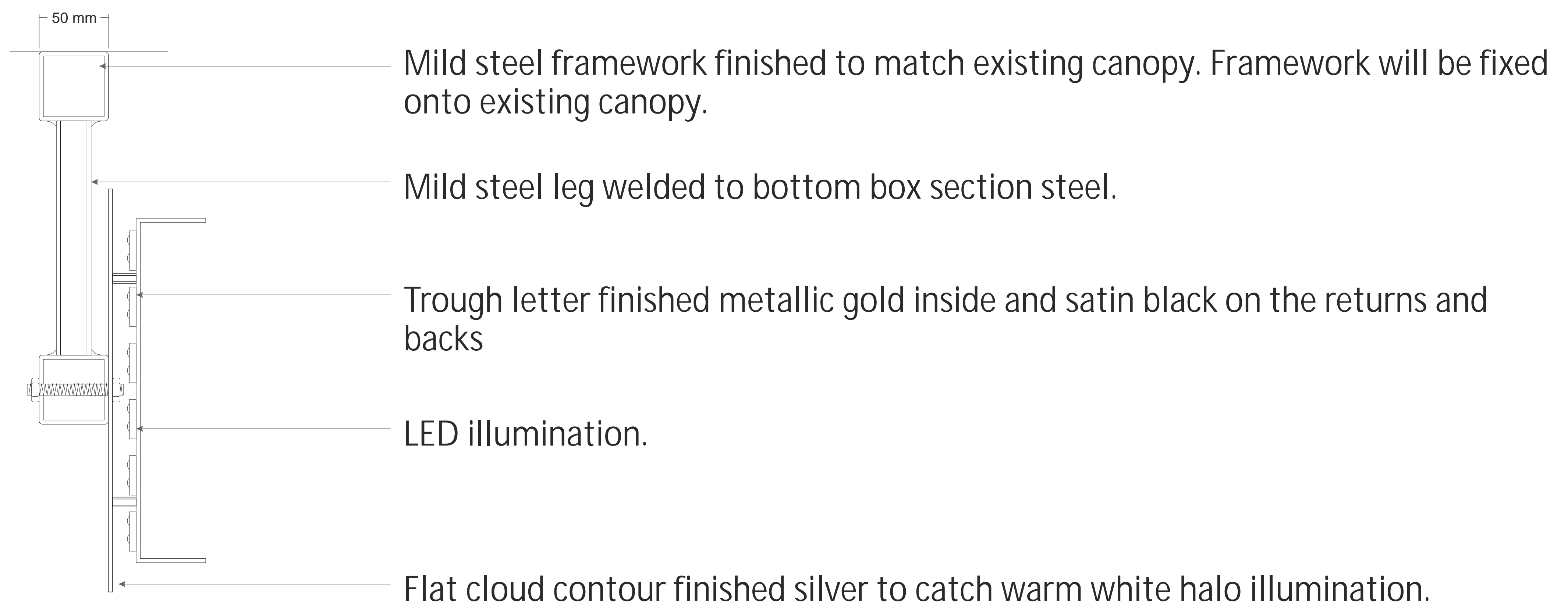
Section for side signs. 1:2 @ A0
