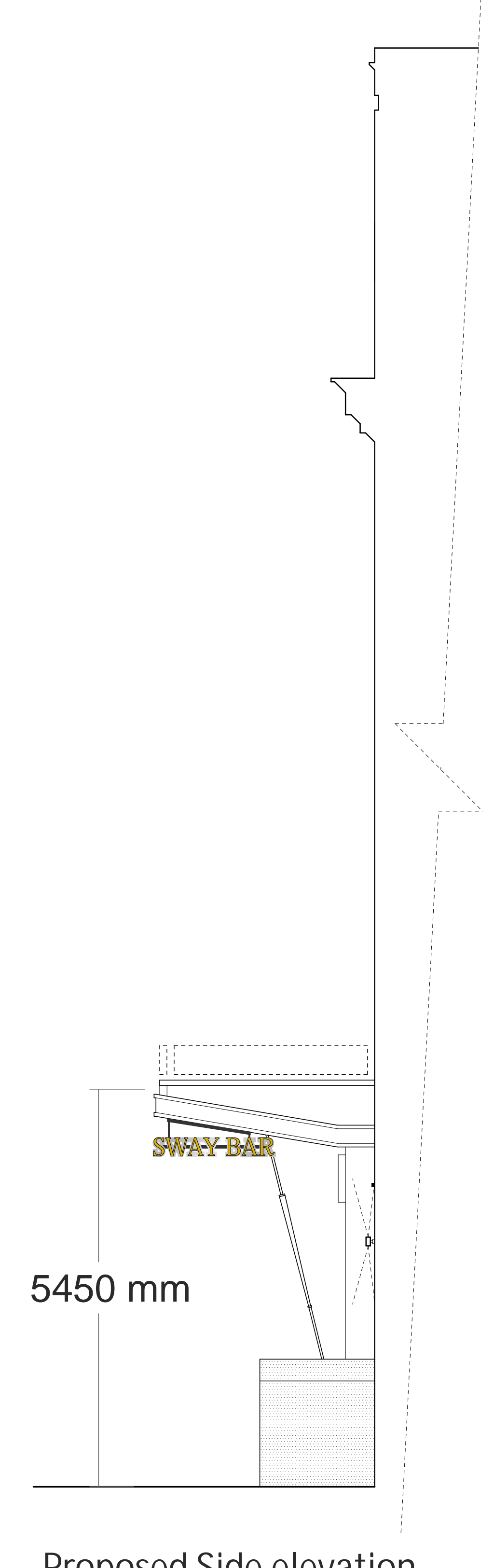
Proposed Side elevation Scale 1: 50 @ A0
