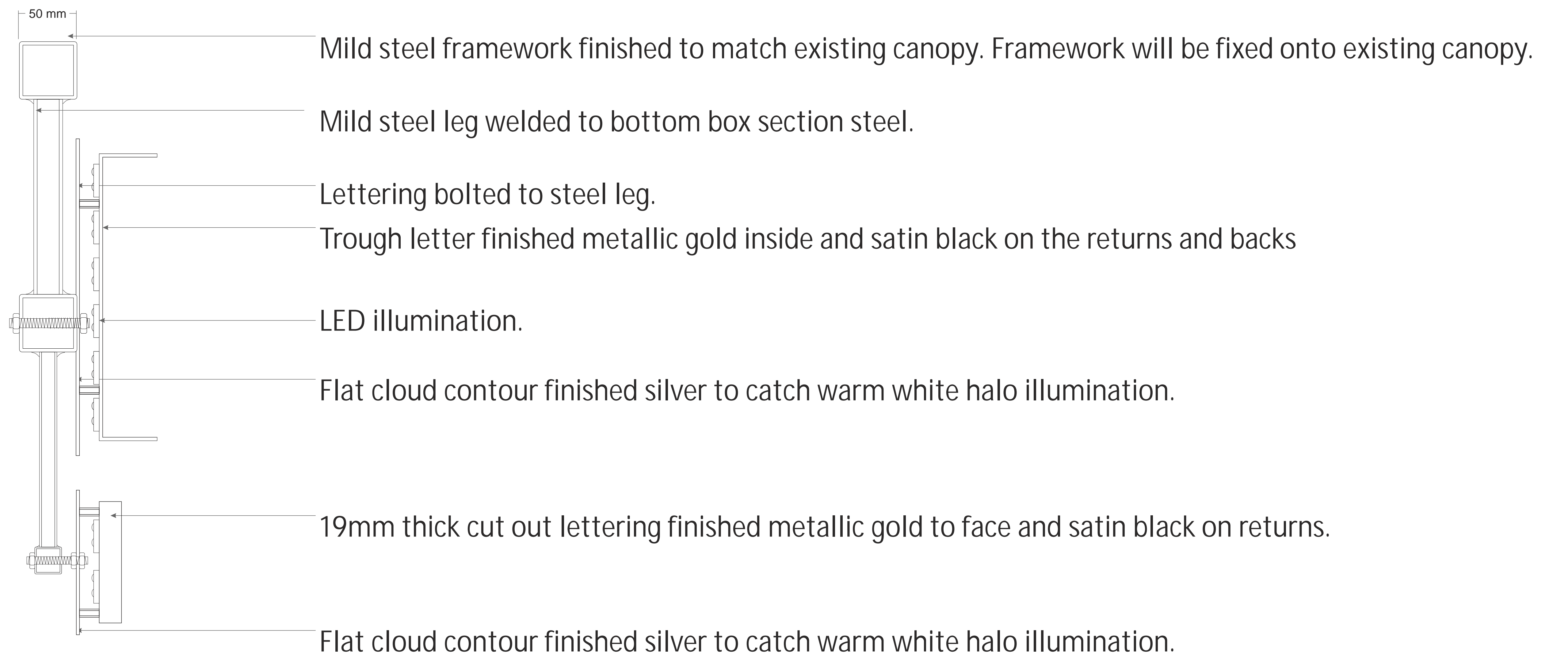
Section for front sign. 1:2 @ A0
