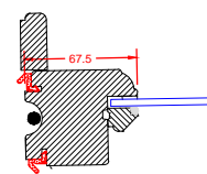
Section B-B Scale-1:5
