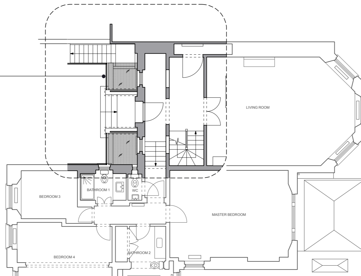
Proposed Upper Ground Floor Plan - Not to scale
