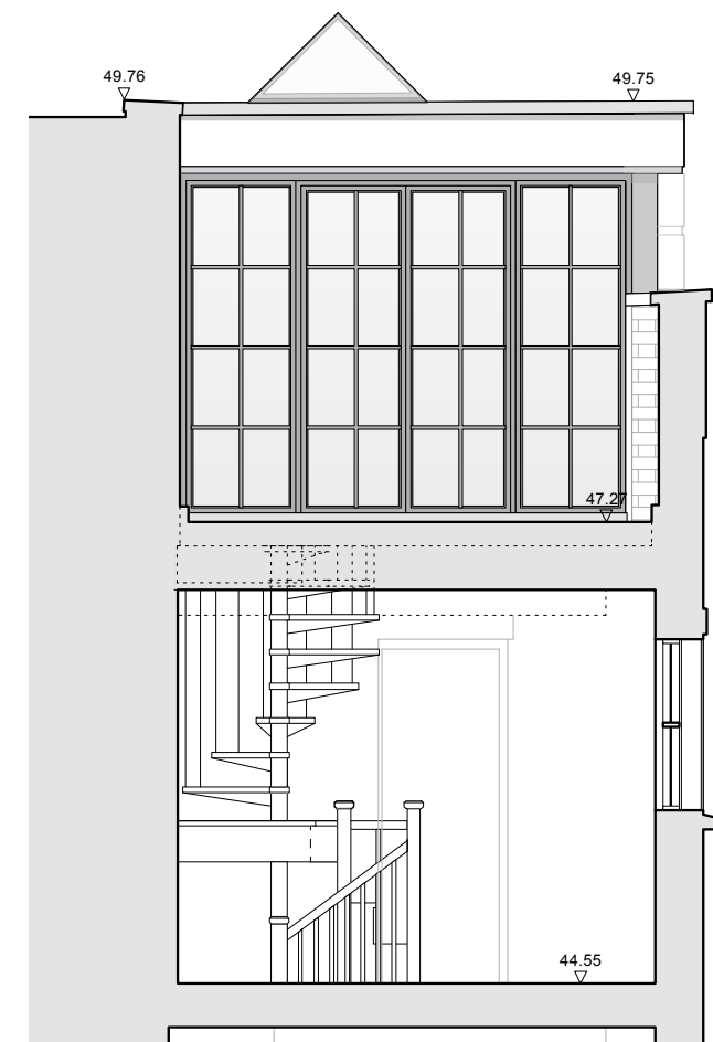
2. SECTION BB
