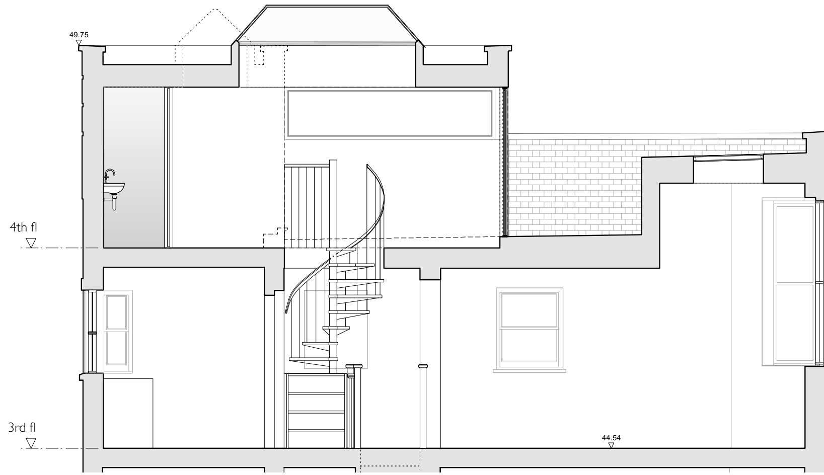
1. SECTION AA
