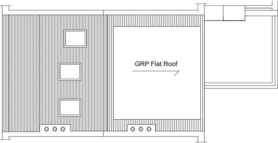
ROOF LAYOUT AS PROPOSED
