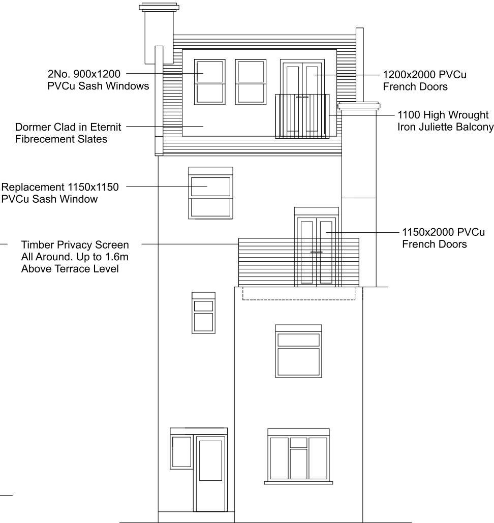
REAR ELEVATION AS PROPOSED
