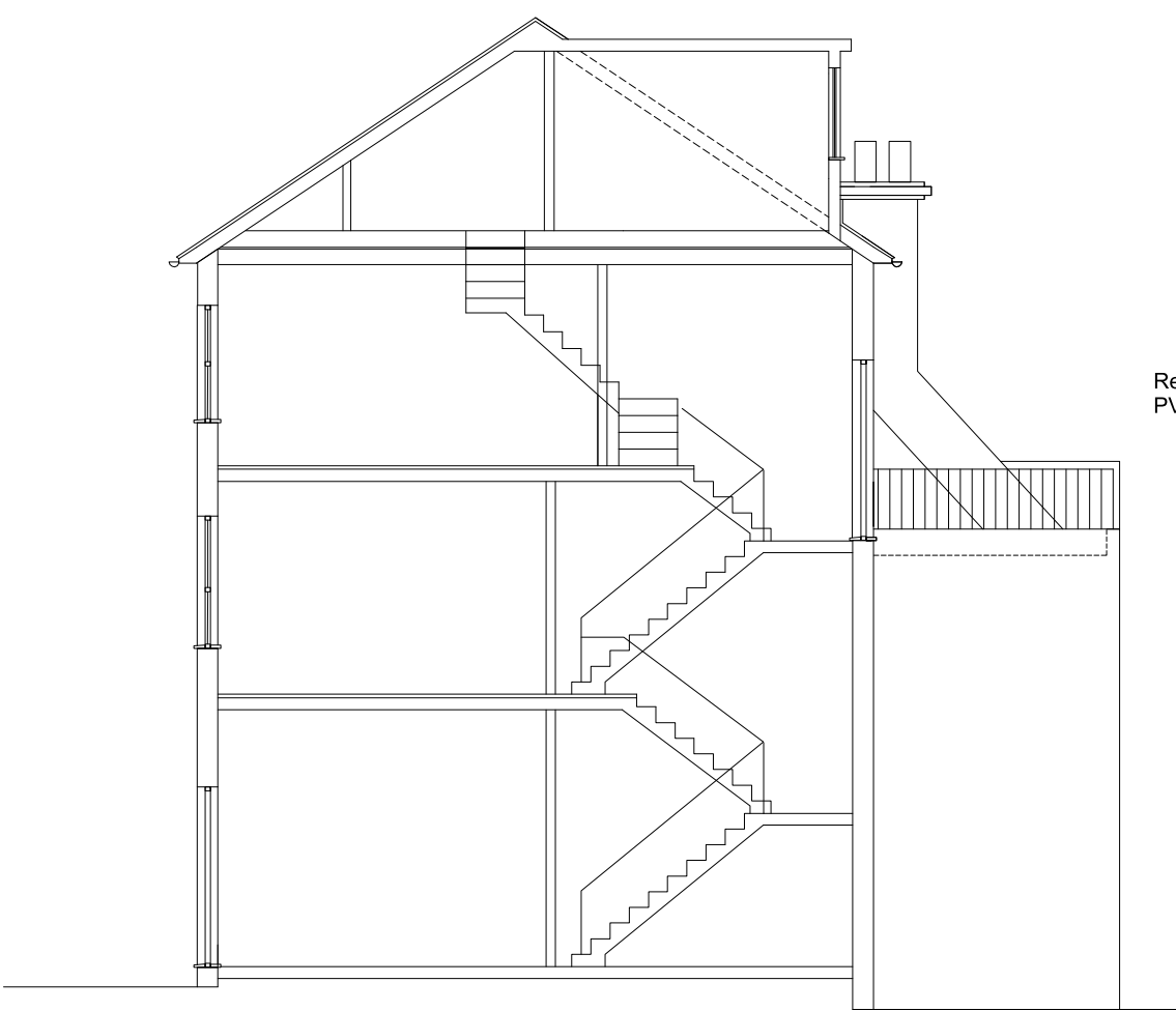
SECTION AS PROPOSED
