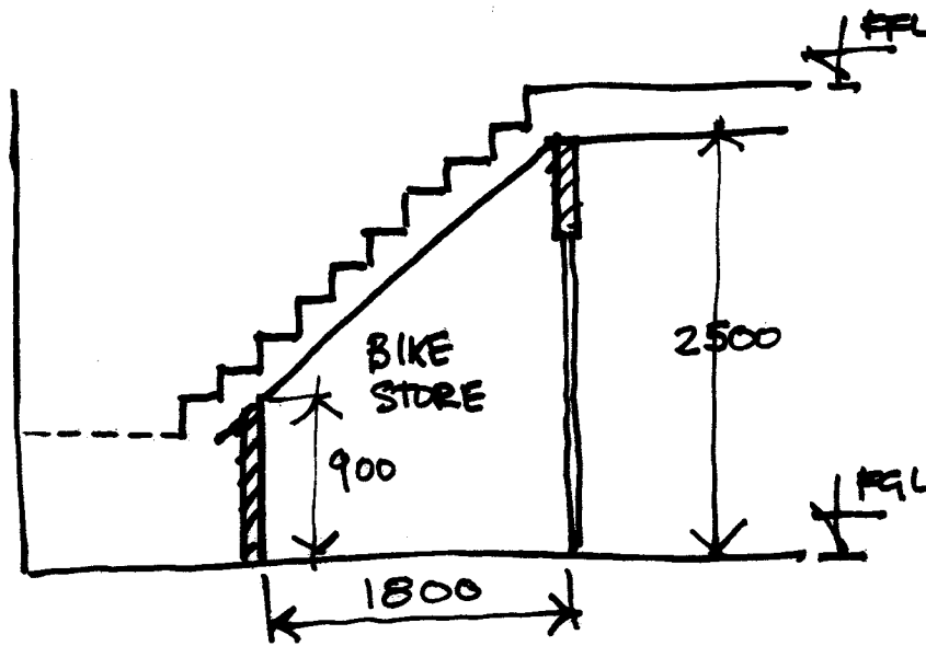
A: SECTION THRO' BIKE STORE FOR FLAT 1
